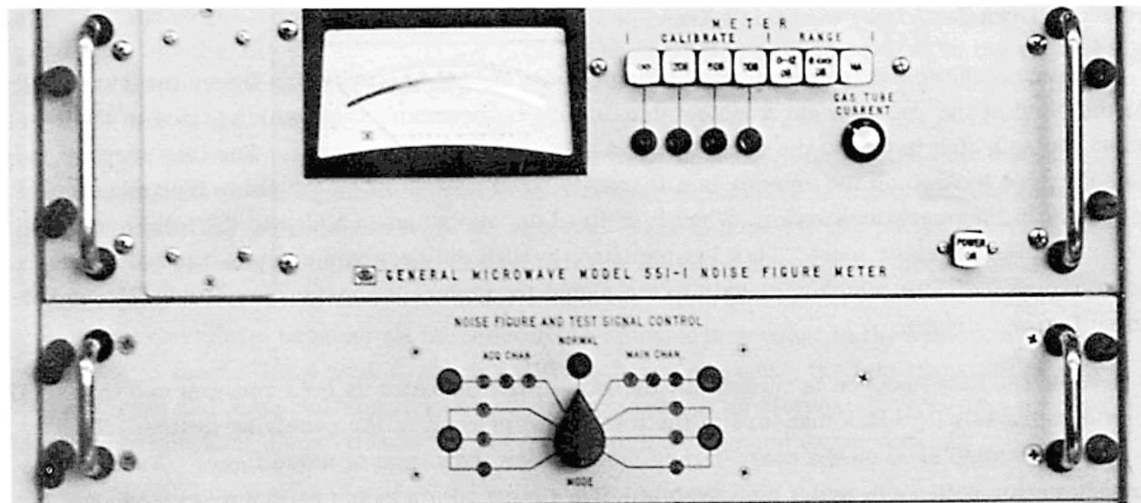
Figure 3—Noise figure and test signal network equipment.
