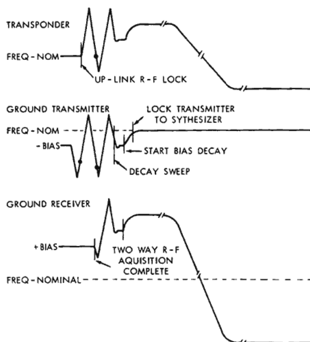
Figure 5—Typical RF acquisition sweep procedure.
