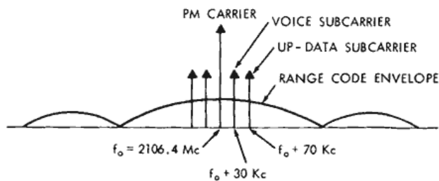
Figure 1—Full up-link spectrum with the range of code, voice, and up-data subcarriers.
