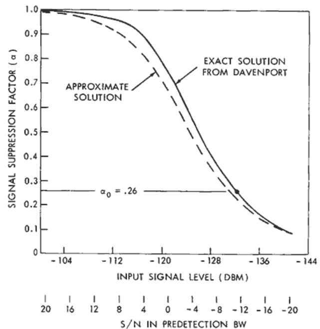
Figure 8—Signal suppression versus input signal level and S/N in predetection BW, when \alpha = \sqrt{1/(1 + 4/\pi N/S)} (approximate) where N equals KTBF (noise power in predetection BW), S equals signal power, B_{L0} equals 400 cps, B_{1F} equals 10 kilocycles, and F_n equals 13db.
