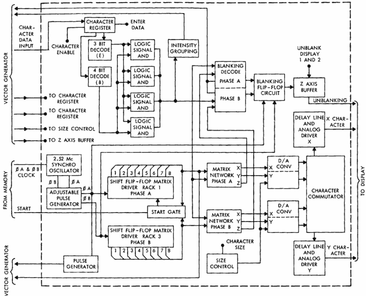
Figure 6—Character generator.
