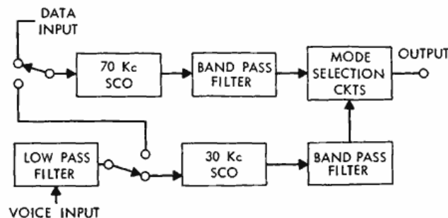
Figure 5—Subcarrier oscillator subsystem.
