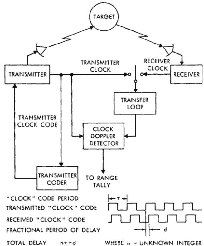
Figure 3—Determination of fractional cycle.
