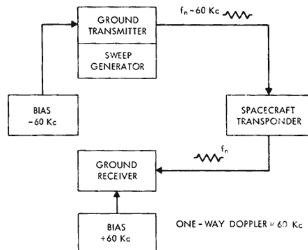
Figure 4—Procedure for acquisition at horizon for an overhead pass using receiver and transmitter bias.
