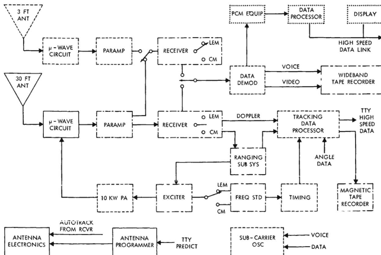
Figure 10—USB system antenna facility primary stations.
