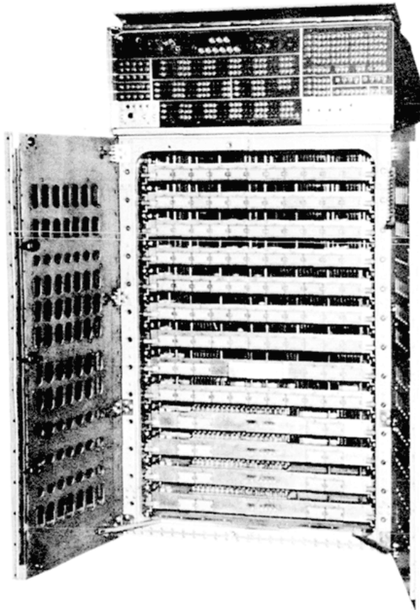
Figure 1—624B modified computer.
