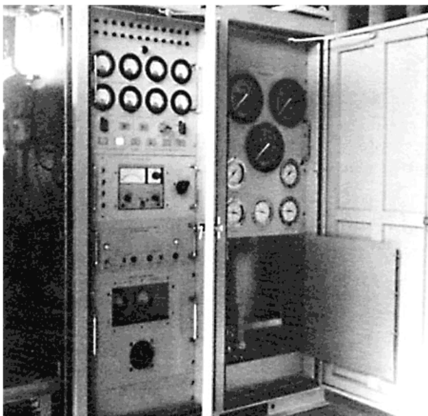
Figure 4—RF enclosure.
