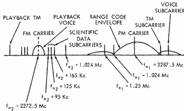
Figure 3—Typical down-link spectrum with a normal PM mode.
