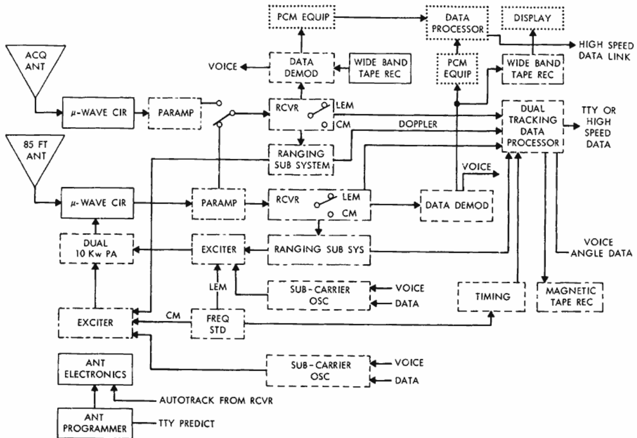
Figure 8—USB system 85-foot antenna facility primary stations.
