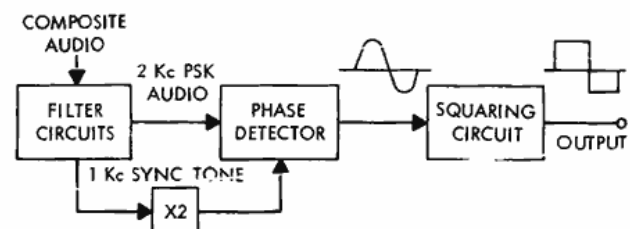
Figure 4—PSK demodulator.
