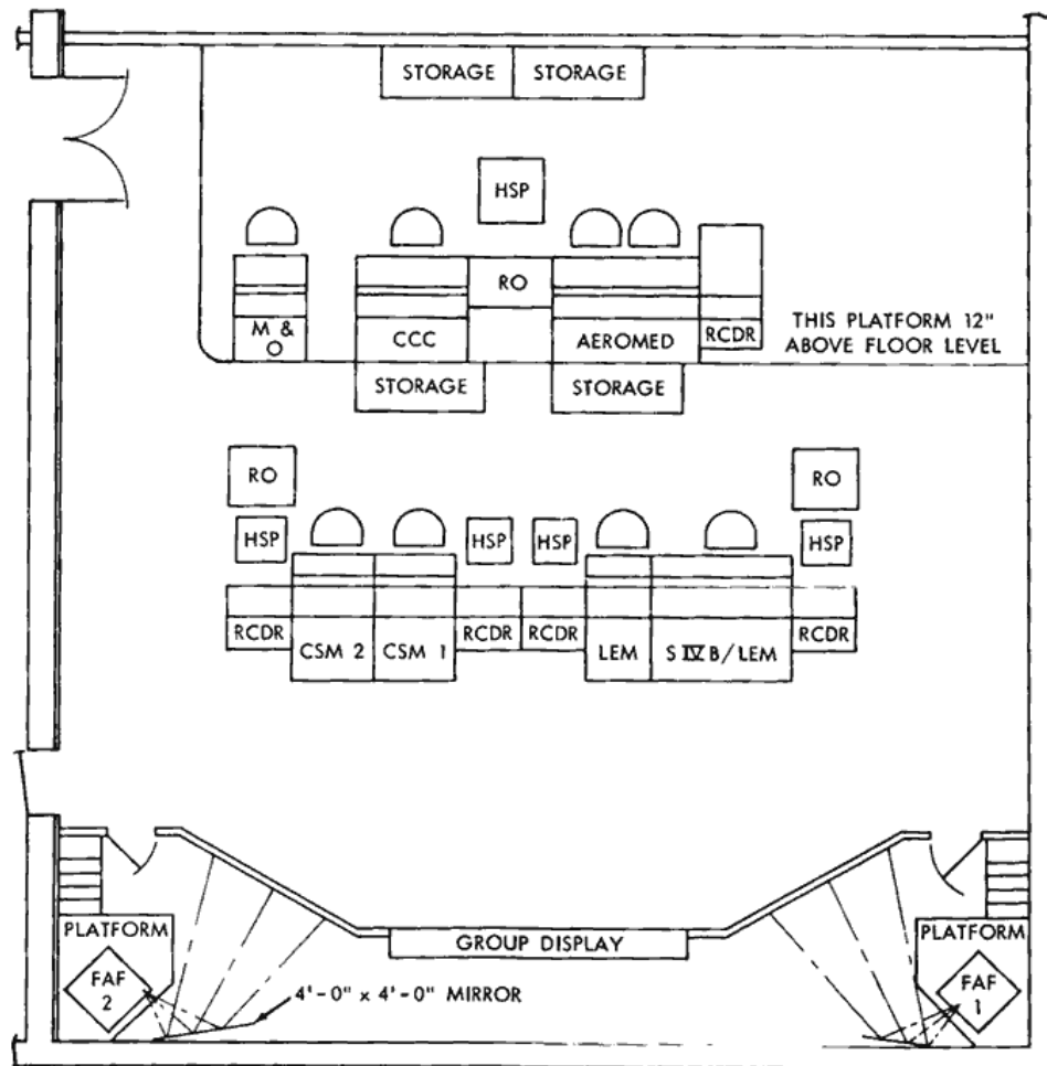
Figure 3—Apollo flight operations room layout.
