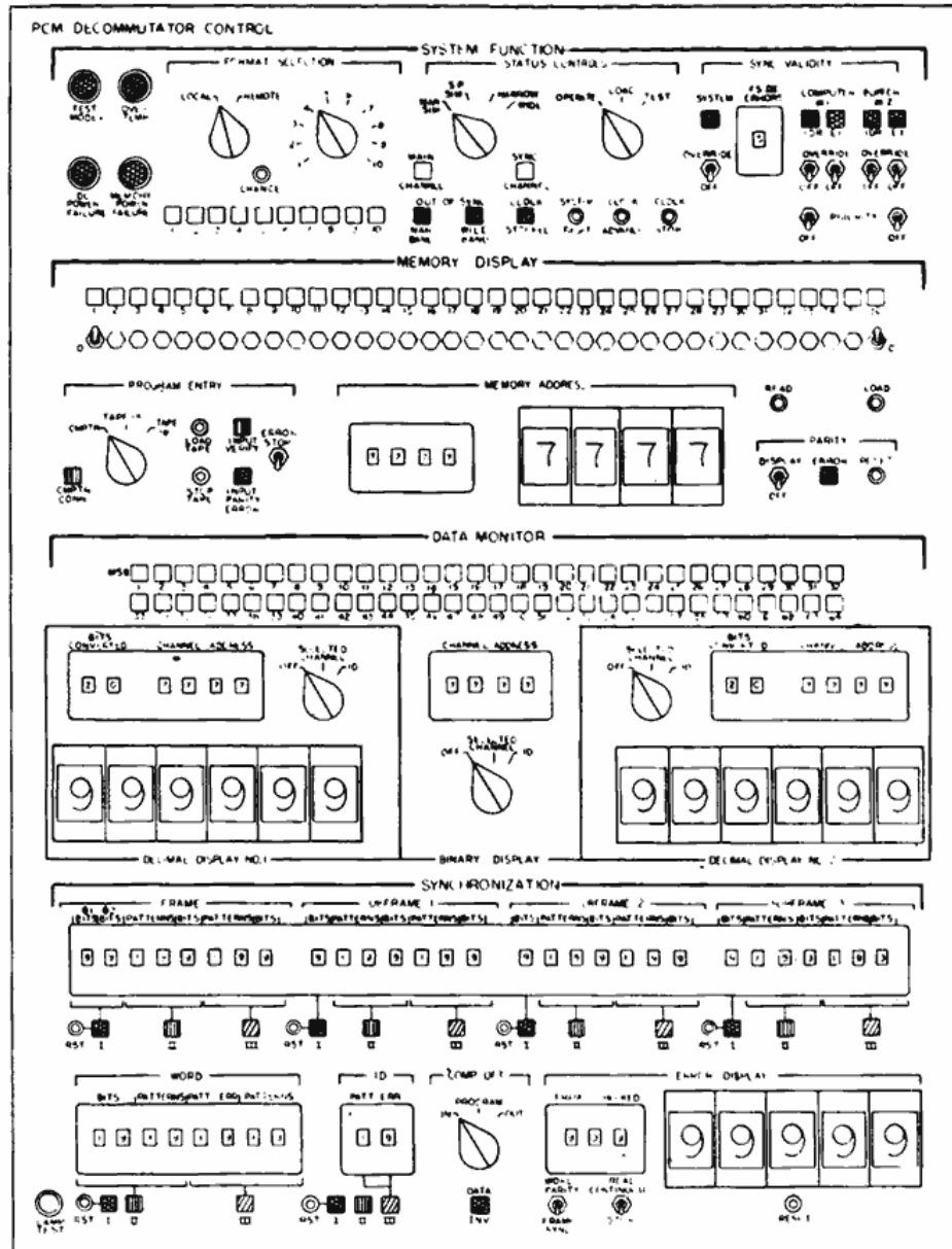
Figure 7—PCM decommutator control panel.
