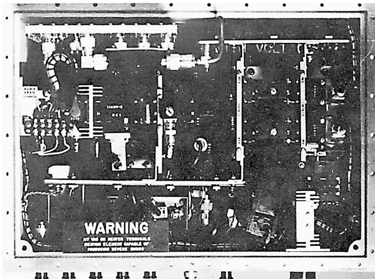
Figure 8—Top view of parametric amplifier.
