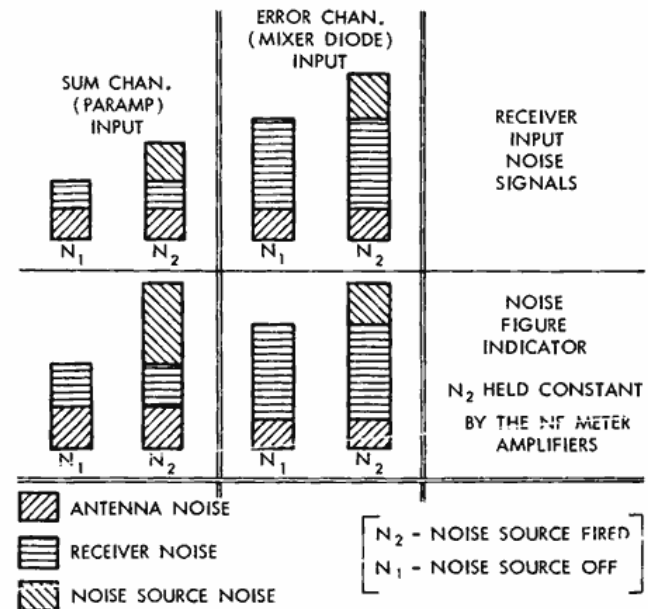
Figure 2—Basic concept of automatic noise figure measurement.
