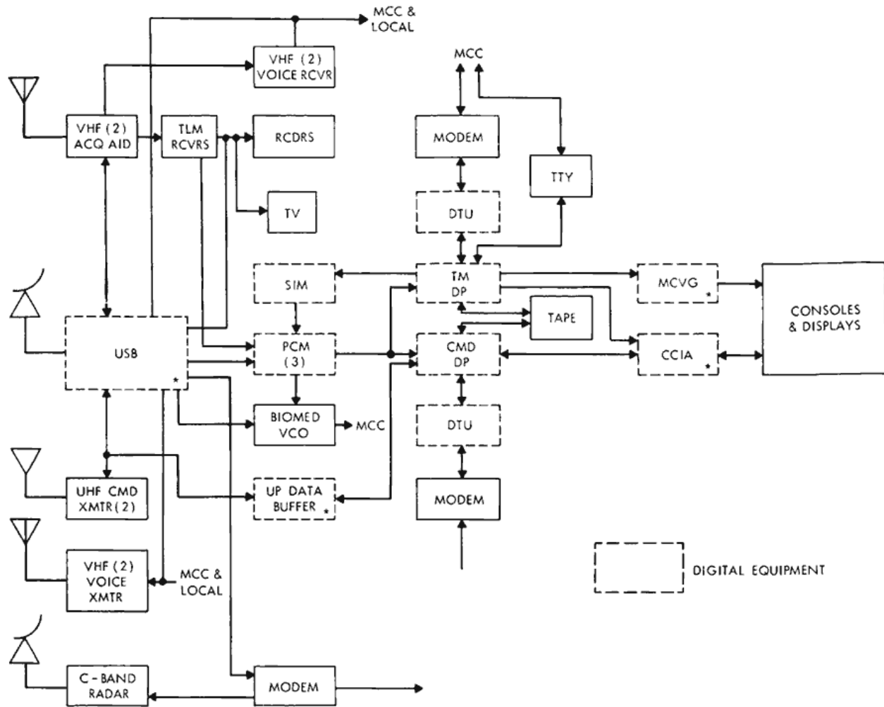
Figure 7—Typical remote site digital equipment block diagram.
