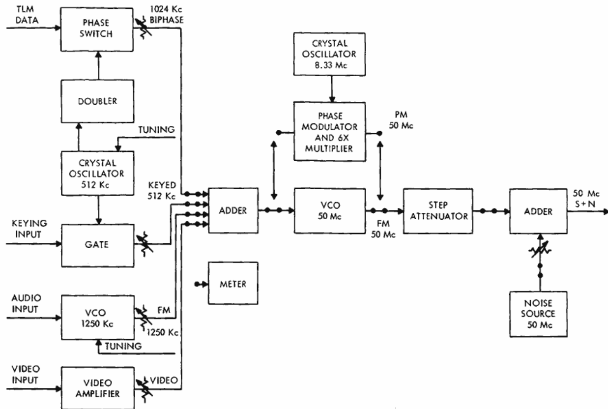
Figure 9—SDDS test system.
