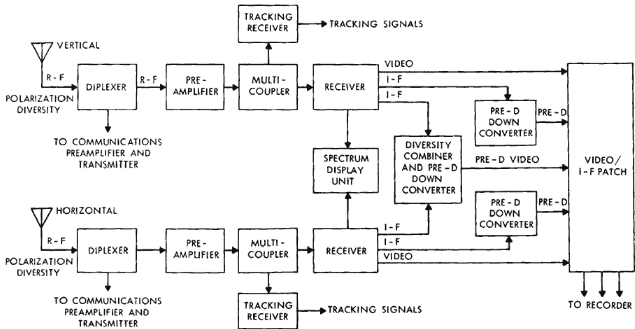
Figure 7—VHF telemetry receiving system block diagram.
