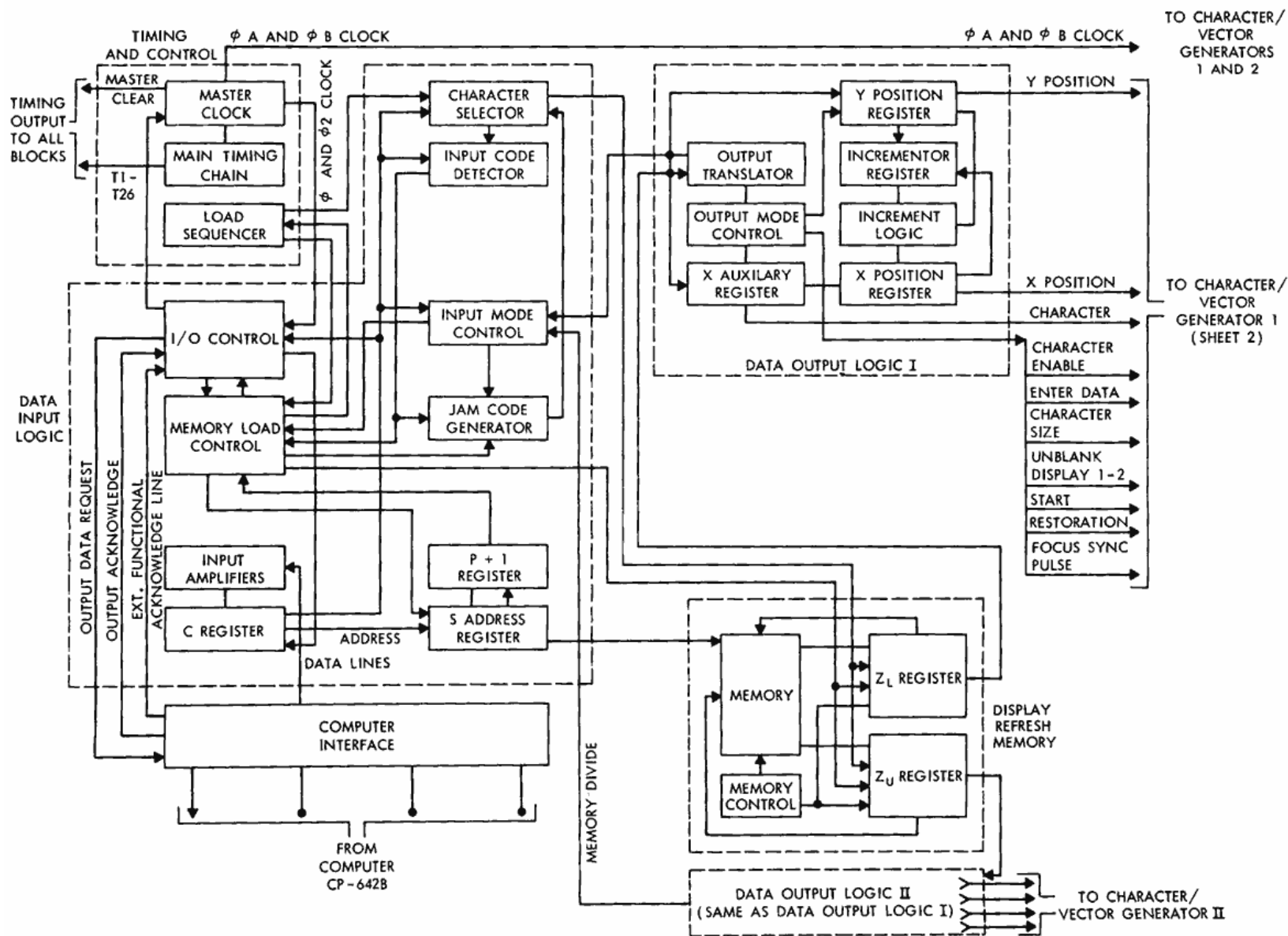
Figure 5—Memory channel block diagram.
