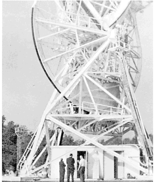
Figure 8—Eighty-five-foot antenna X-wheel structure.
