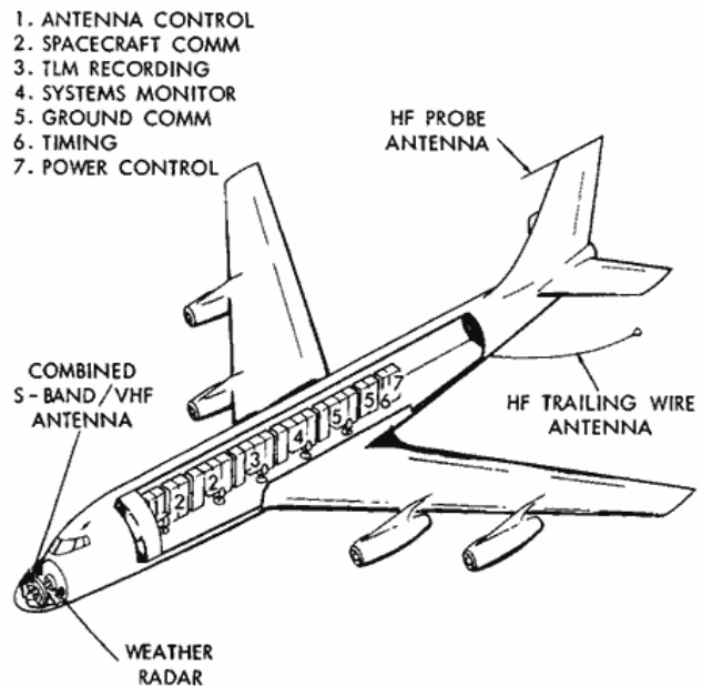
Figure 5—Aircraft equipment arrangement.
