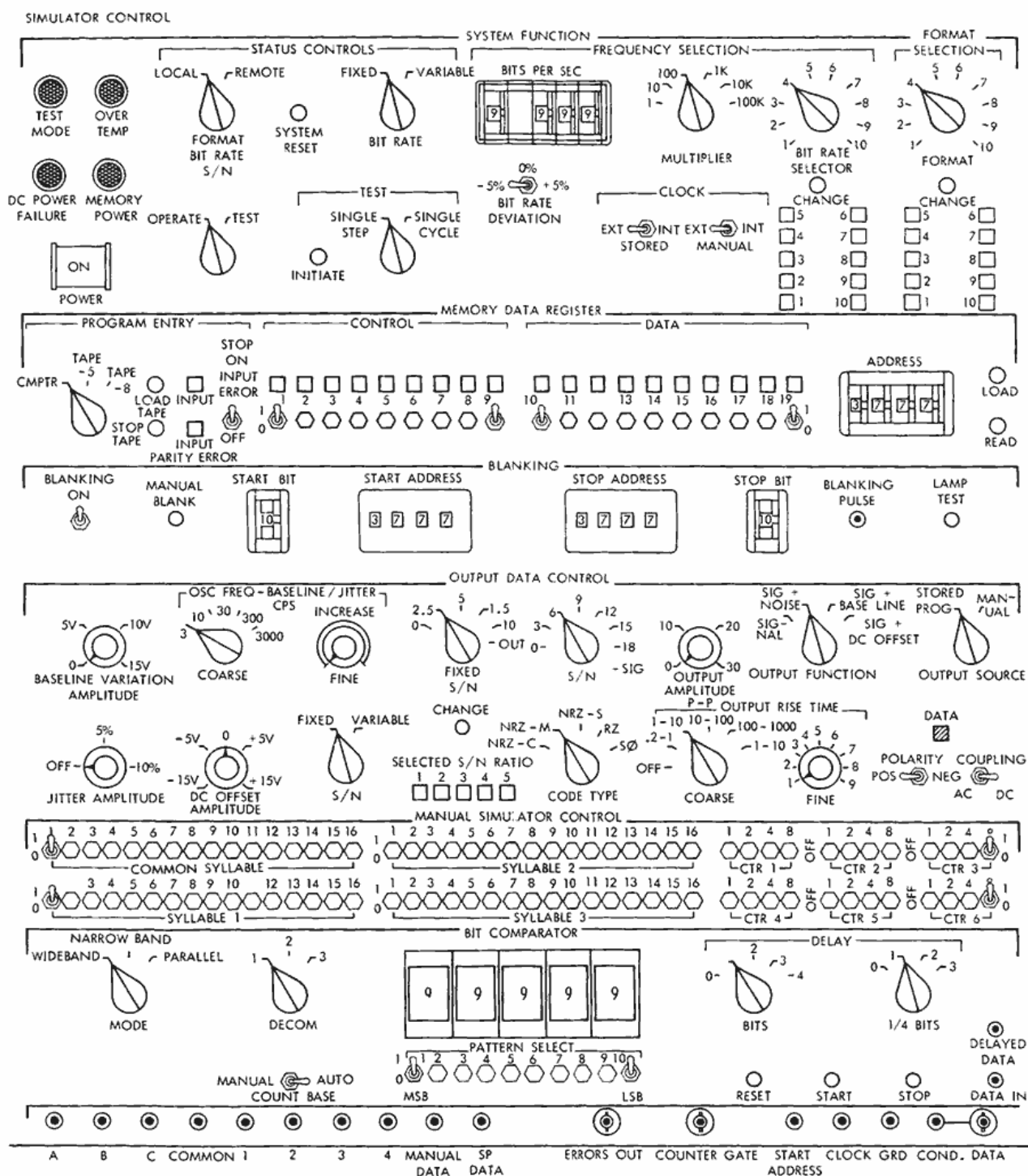
Figure 11—PCM stored program simulator control panel.
