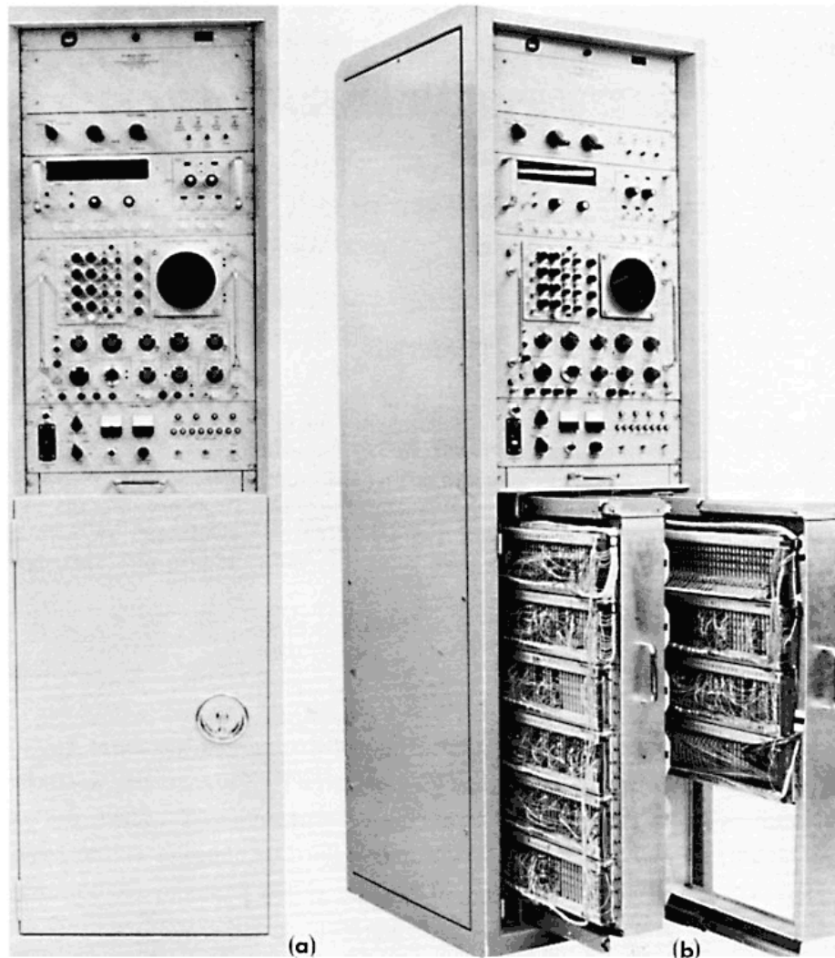
Figure 7—(a) Ranging subsystem Mark I (closed). (b) Ranging subsystem Mark I (open).
