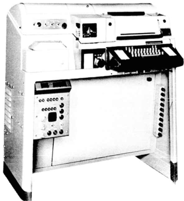
Figure 4—UNIVAC teletype adapter and modified ASR-28 set.
