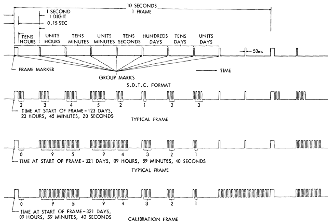
Figure 8—Apollo format serial decimal time code.
