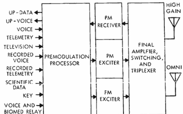
Figure 5—Diagram of basic CSM Unified S-Band System.
