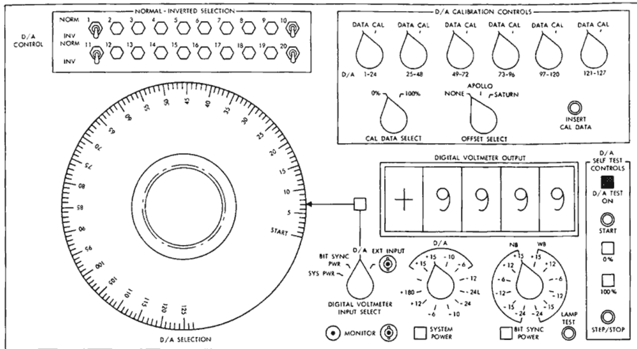
Figure 8—D/A control panel.
