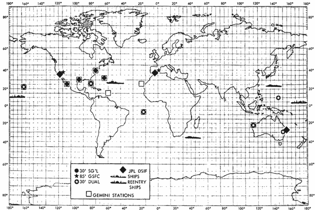
Figure 6—Apollo USB network.
