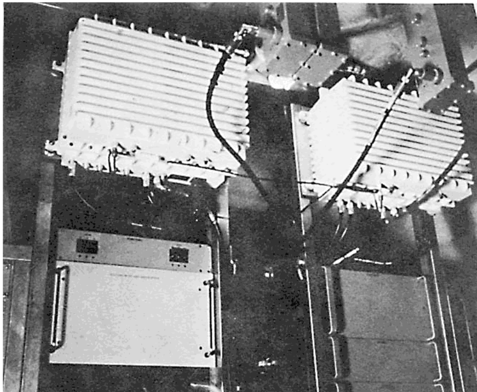
Figure 11—Main channel and acquisition parametric amplifiers mounted in wheelhouse of antenna.
