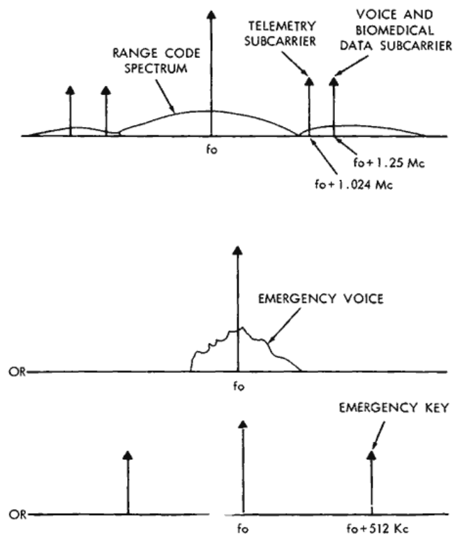
Figure 1—PM spectra of frequency-modulated carriers.
