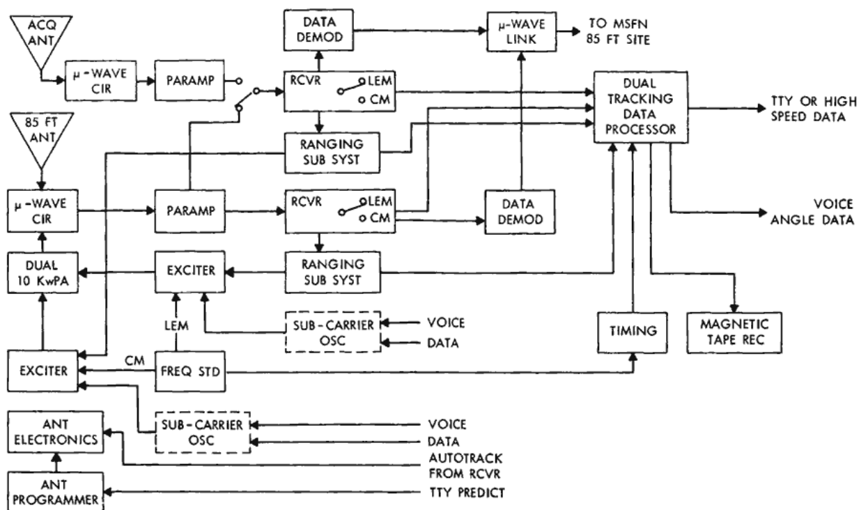
Figure 9—USB system 85-foot antenna facility backup station.
