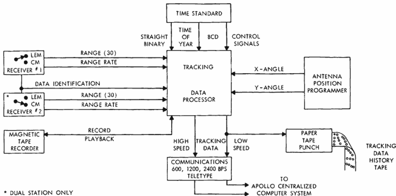
Figure 5—USB system tracking data processor.
