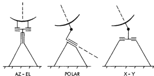
Figure 1—Antenna mounts.
