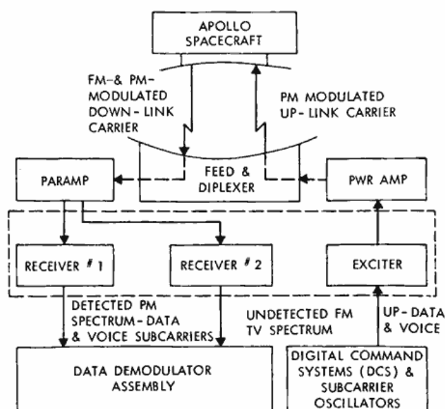
Figure 3—Two-way communications function.
