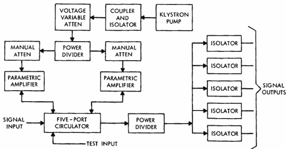
Figure 5—Block diagram of parametric amplifier.
