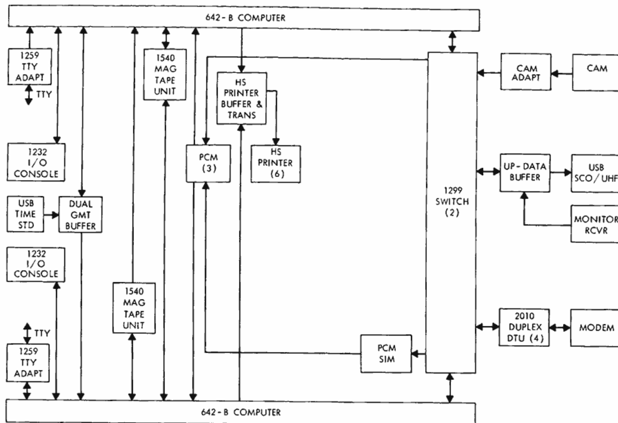
Figure 11—Block diagram of site without flight control console.
