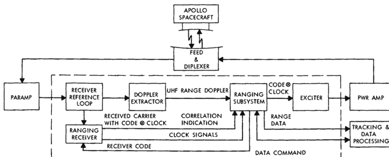
Figure 5—Ranging function.
