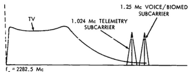
Figure 5—FM down-link spectrum.
