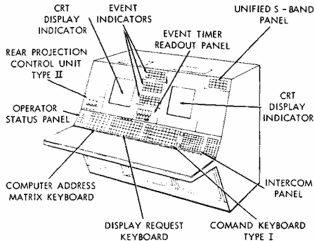
Figure 14—Command communicator console.
