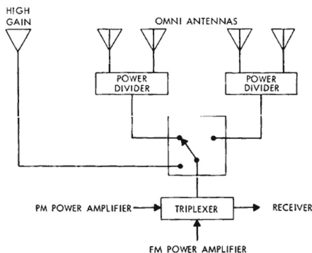
Figure 9—CSM S-band antenna system.
