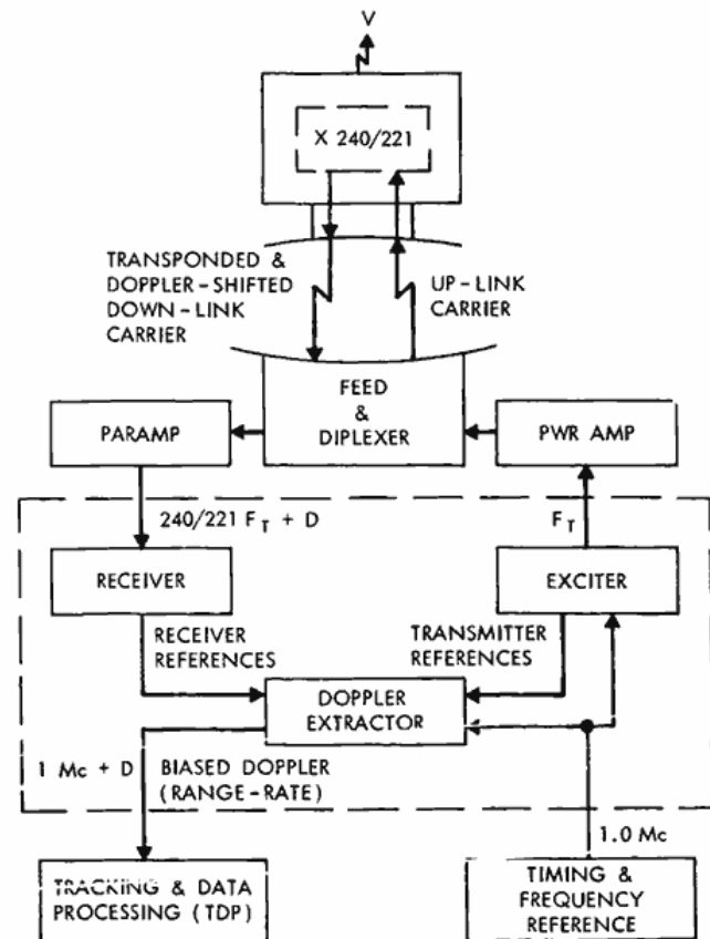
Figure 2—Doppler extraction function.
