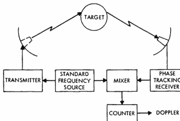
Figure 2—Doppler measurement by coherent CW radar.
