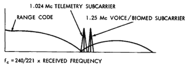
Figure 3—Full down-link PM spectrum.
