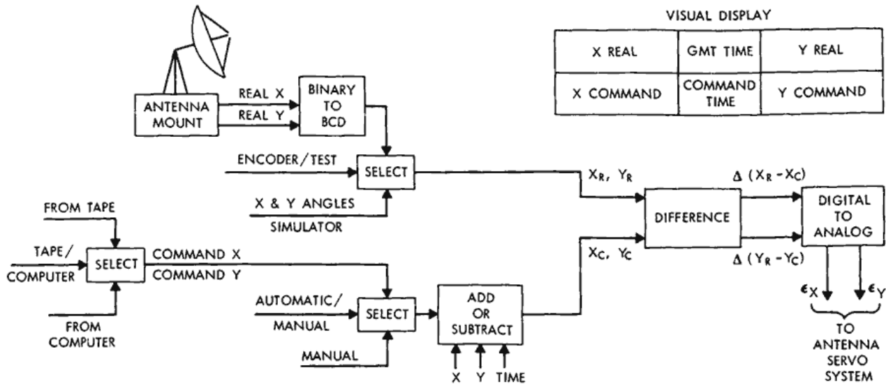
Figure 2—Antenna position programmer.
