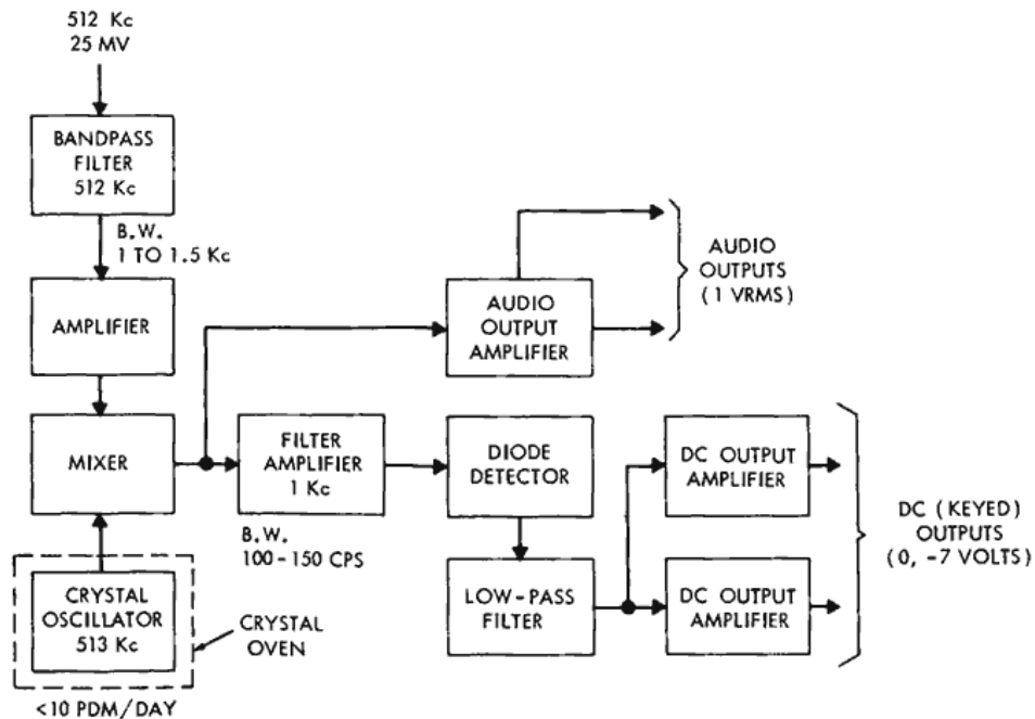
Figure 8—AM key demodulator.
