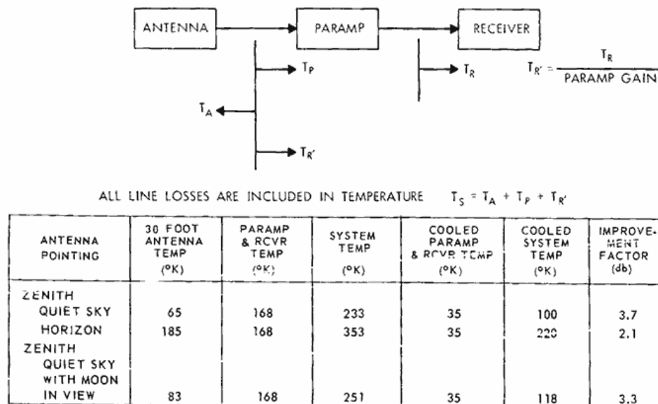
Figure 4—Antenna, parametric amplifier, and receiver circuits.
