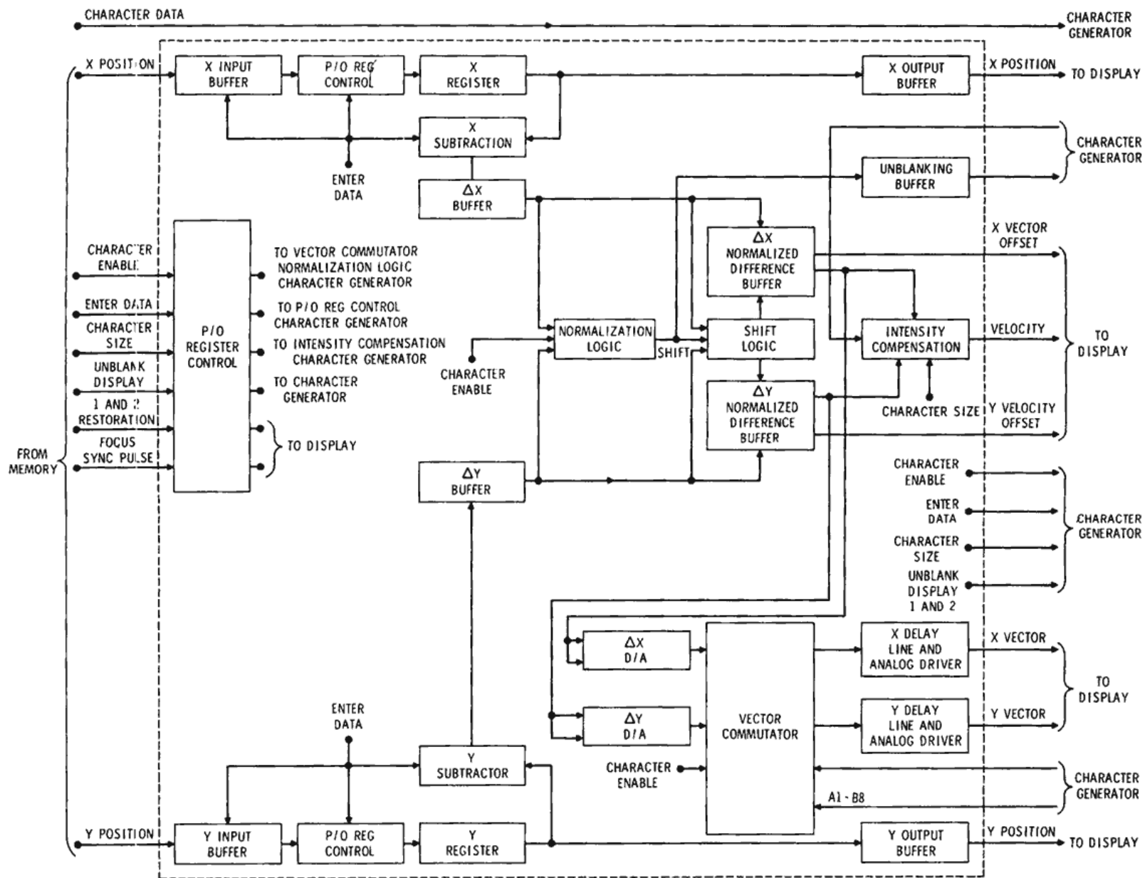
Figure 8—Vector generator.
