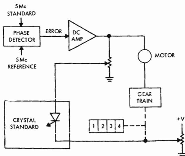
Figure 2—Frequency control loop.
