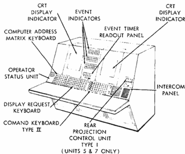
Figure 15—Spacecraft systems console.
