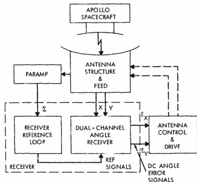
Figure 4—Angle tracking function.
