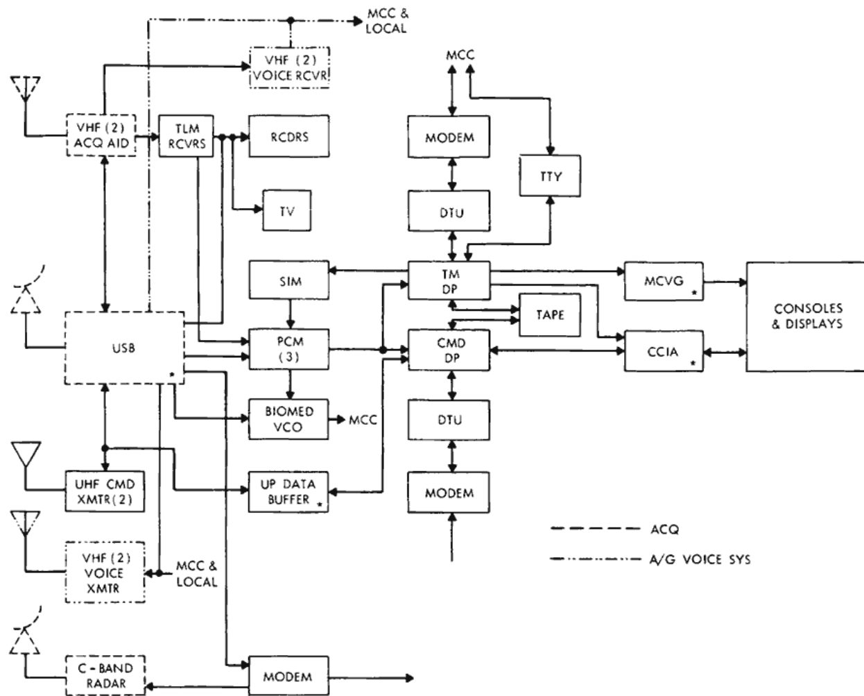
Figure 5—Typical remote site acquisition block diagram.
