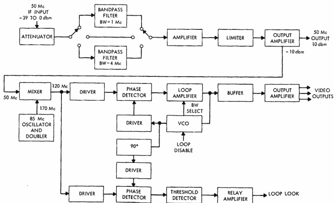
Figure 5—Carrier frequency demodulator.
