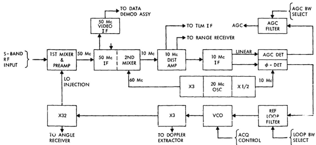
Figure 6—Receiver reference loop (typical).
