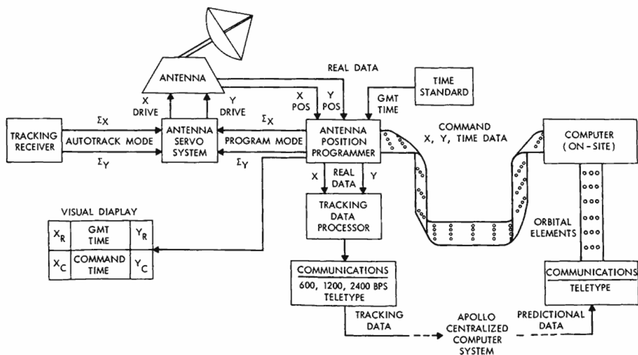
Figure 1—USB system antenna position programmer.
