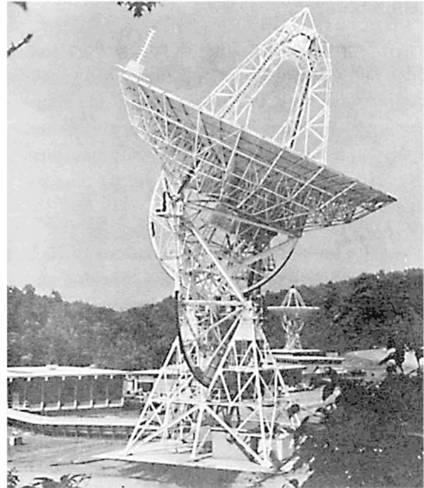
Figure 6—Eighty-five-foot antennas at Rosman.
