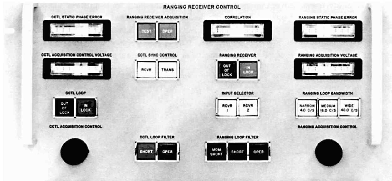
Figure 12—Ranging receiver control.
