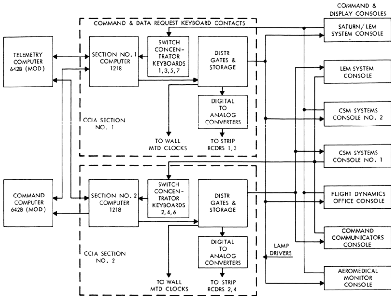
Figure 7—Block diagram - console computer interface adapter.
