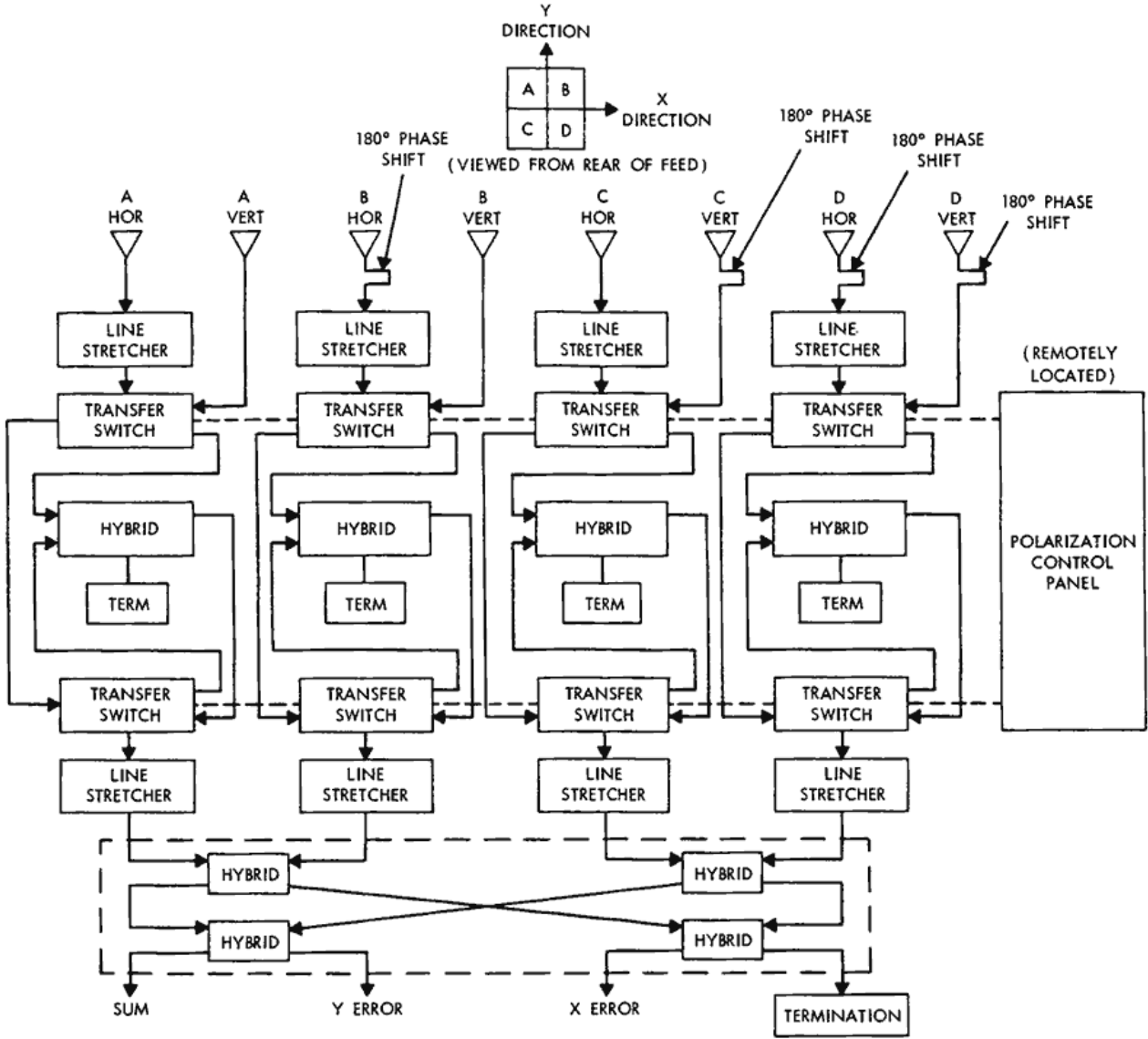
Figure 5—Acquisition antenna, block diagram.
