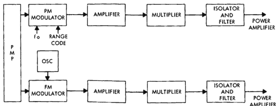
Figure 7—Basic configuration of transmitter PM and FM exciters.
