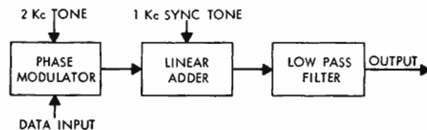
Figure 3—PSK modulator.
