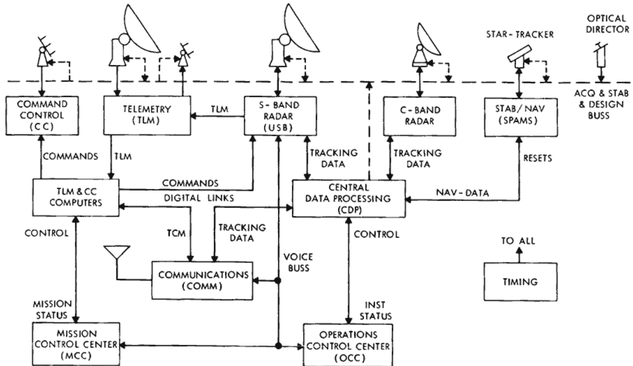
Figure 9—Block diagram of Apollo ships instrumentation systems.
