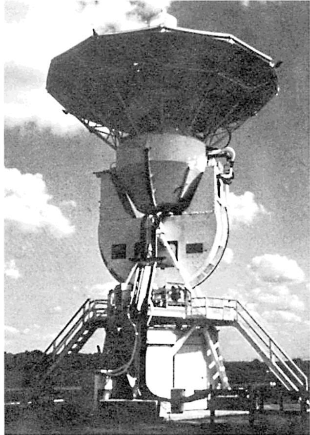
Figure 12—Antenna installation.
