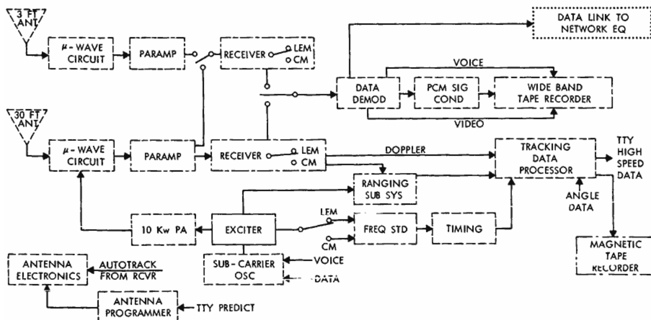
Figure 7—USB system 30-foot antenna facility.
