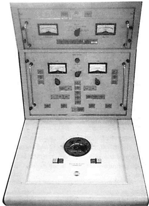
Figure 8—Servo control unit in relation to ball tracker.
