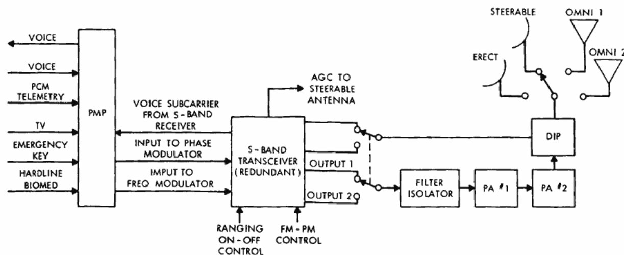
Figure 1—Block diagram of LEM S-band system.
