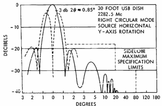
Figure 4—Typical receiving patterns.
