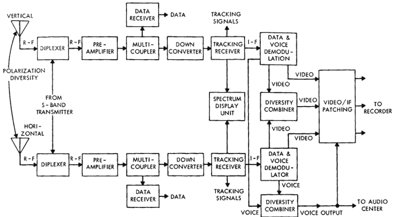
Figure 6—S-band receiving system block diagram.
