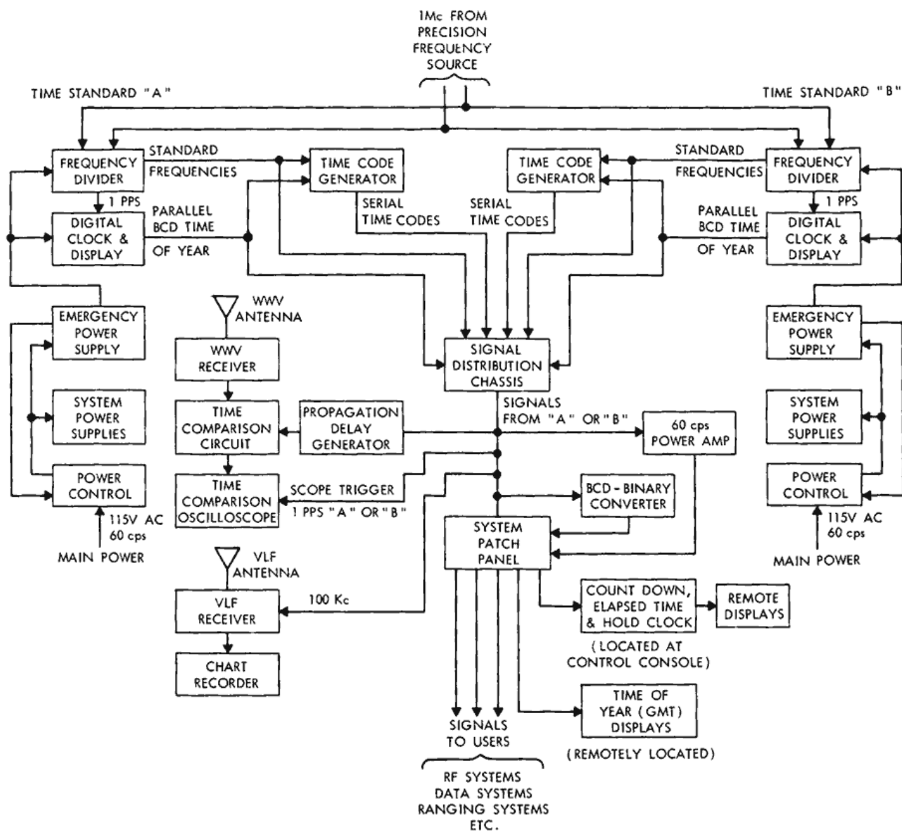
Figure 3—Time standard block diagram.
