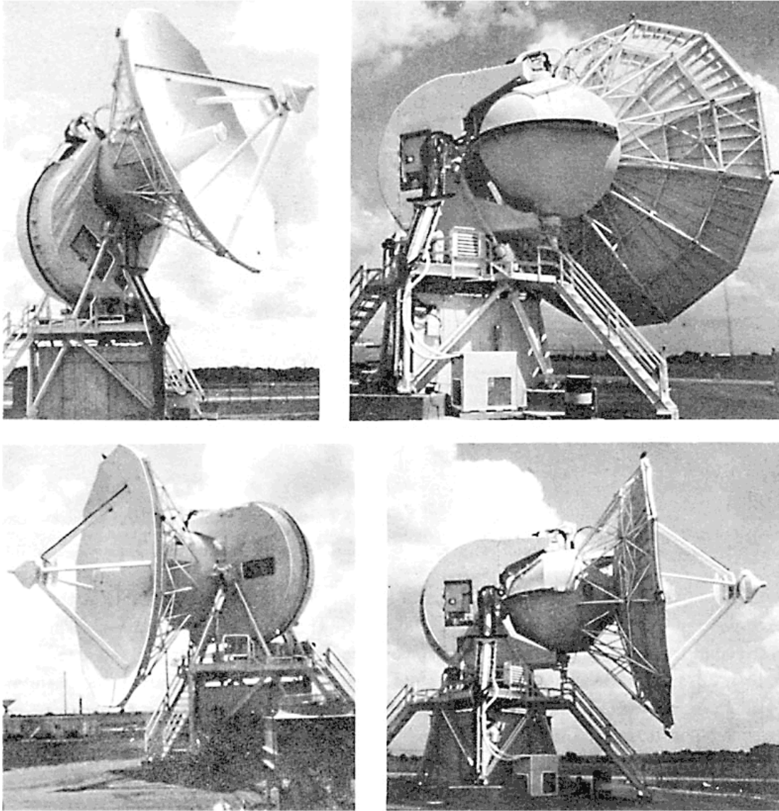
Figure 4—Thirty-foot antenna, axis movements.
