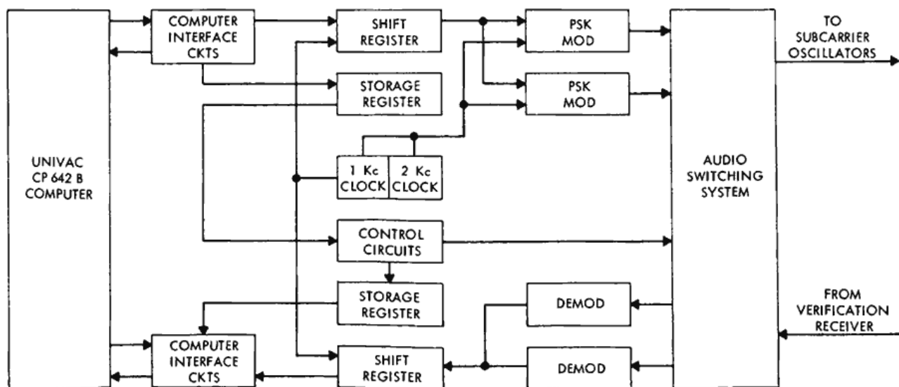
Figure 2—Up-data buffer modem.
