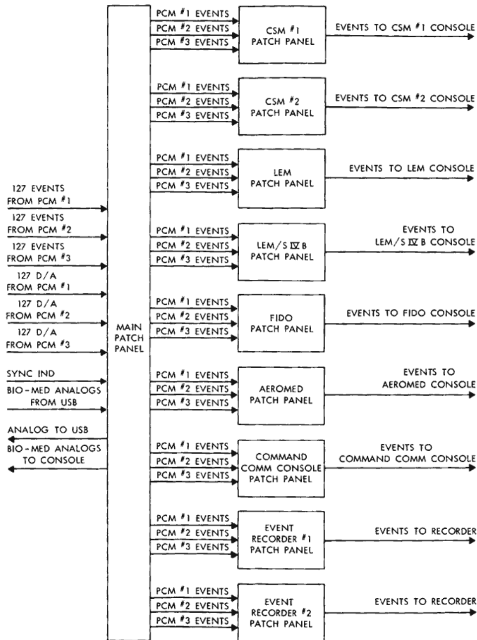
Figure 12—Block diagram of decommutation distribution system.
