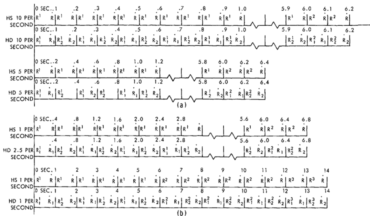
Figure 8—Range and range rate recording - high speed.
