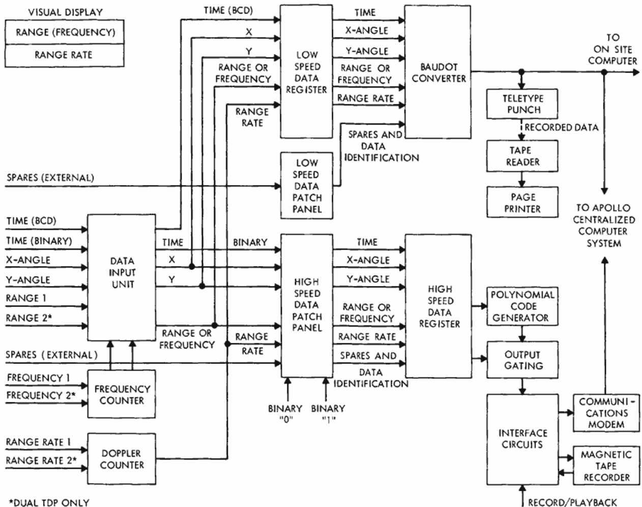
Figure 6—Tracking data processor.
