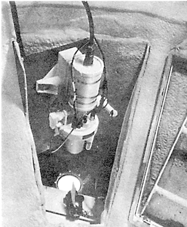
Figure 5—Thirty-foot antenna, optical boresight package.
