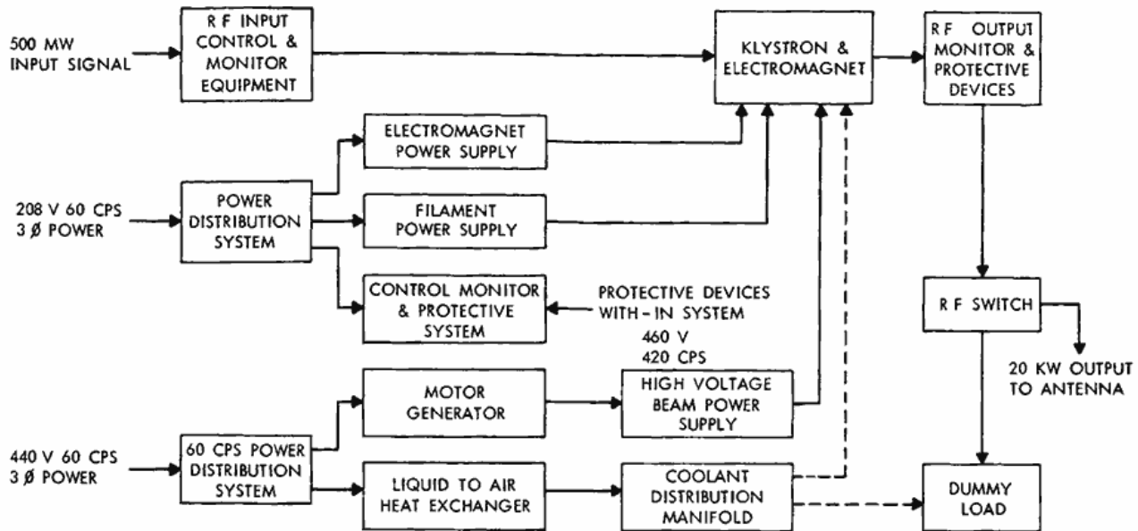
Figure 1—Power amplifier system block diagram.
