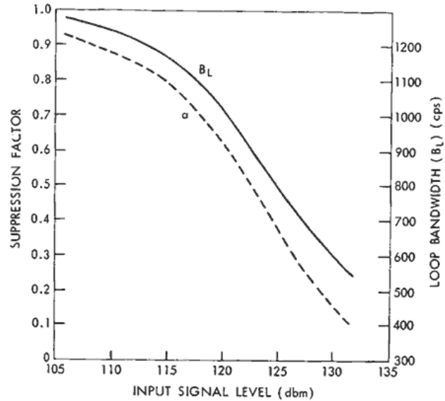
Figure 7—Loop bandwidth and suppression factor versus input signal level, where \alpha = (1 + 4/\pi N/S)^{-1/2} , B_L = B_{L0} (1/3 + 2/3\alpha_0) , \alpha_0 = 0.242 , and B_{L0} = 400 cps.
