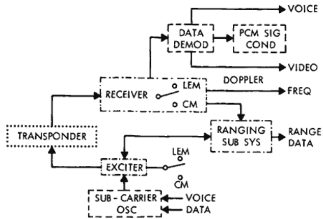
Figure 11—USB system test unit.
