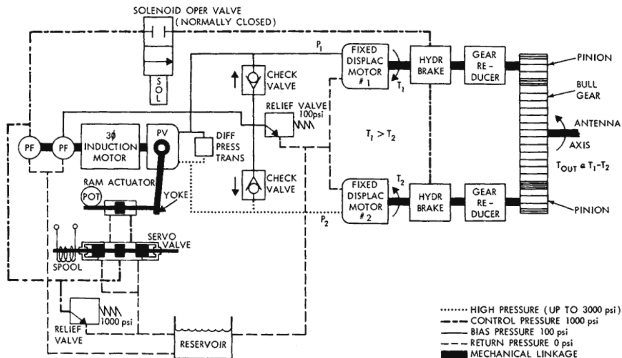
Figure 6—Schematic of hydraulic drive system with drive signal to servo valve reversed.
