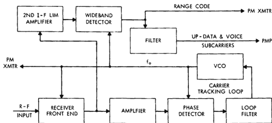
Figure 6—Diagram of CSM S-band receiver.
