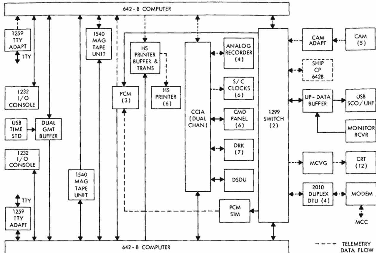
Figure 12—Telemetry data flow.
