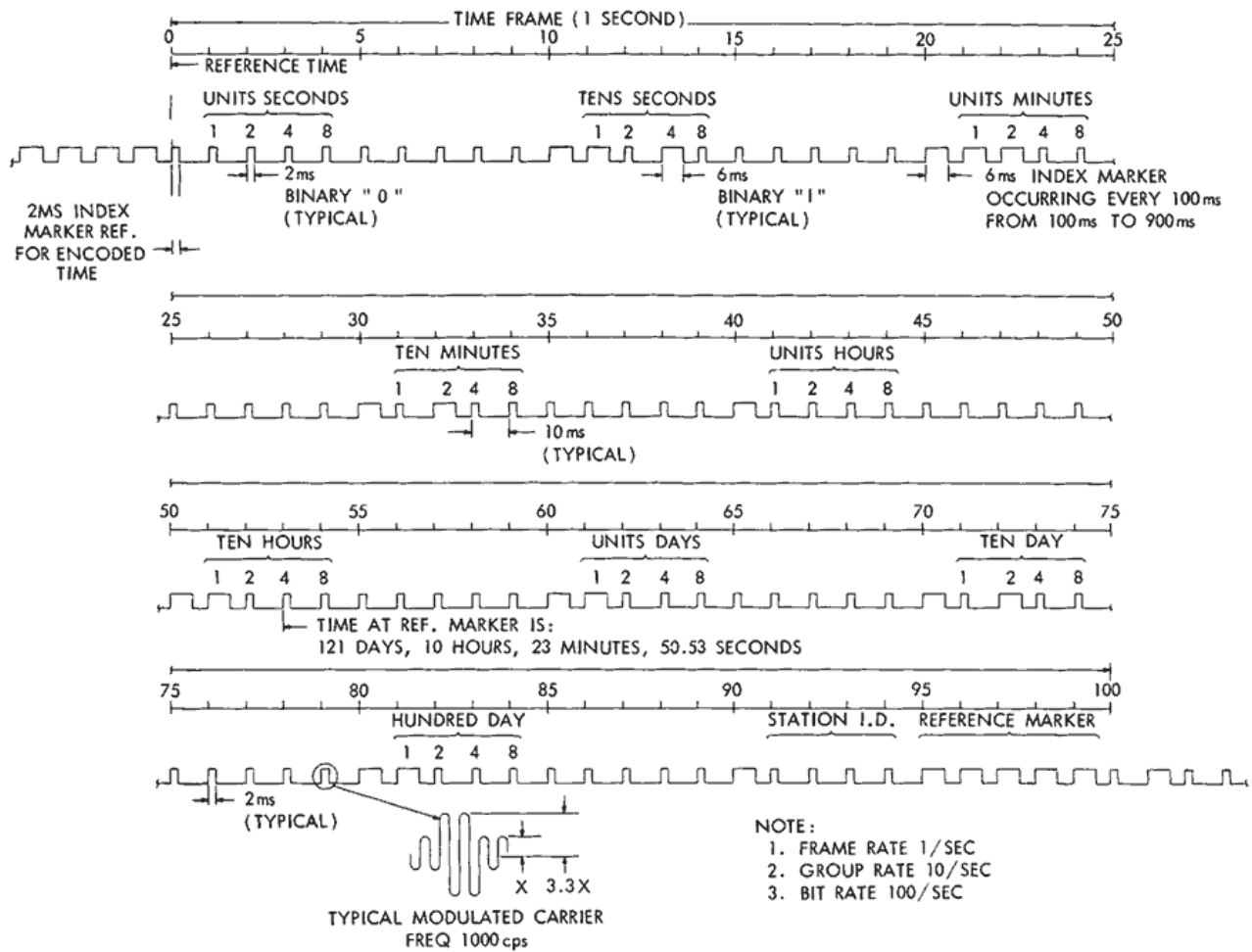
Figure 4—NASA 1/second binary time code.
