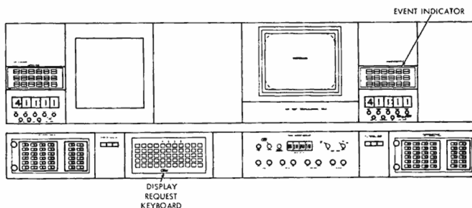
Figure 17—Panels of Aero-Medical console.
