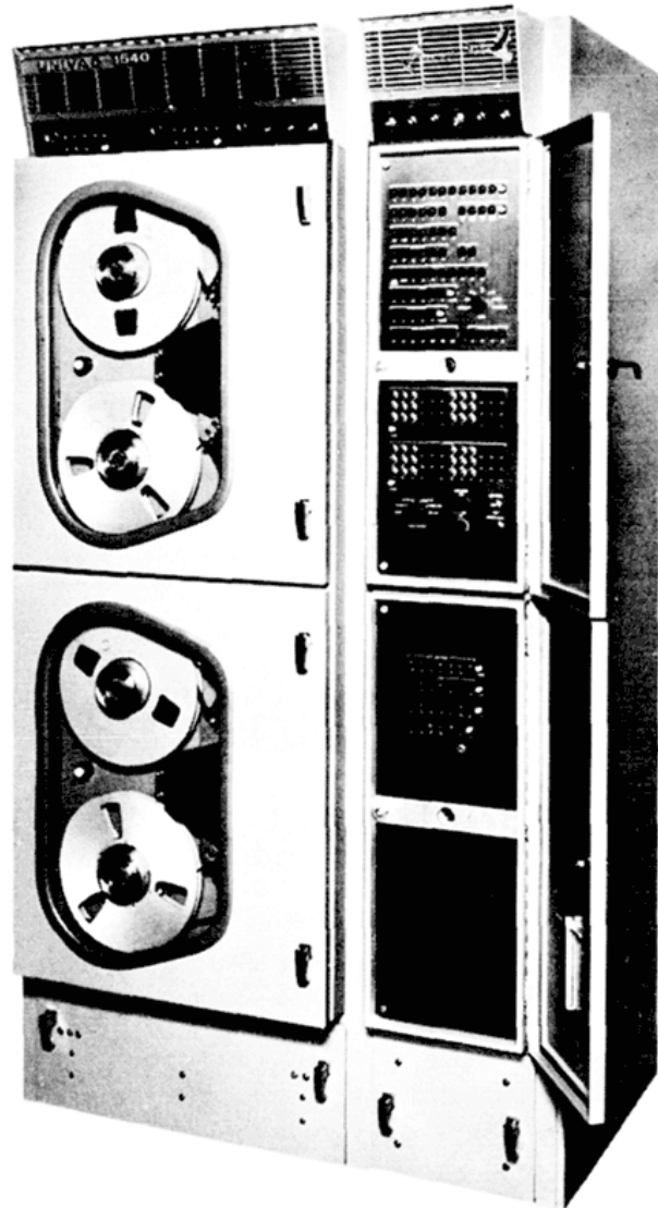
Figure 2—1540 magnetic tape unit.
