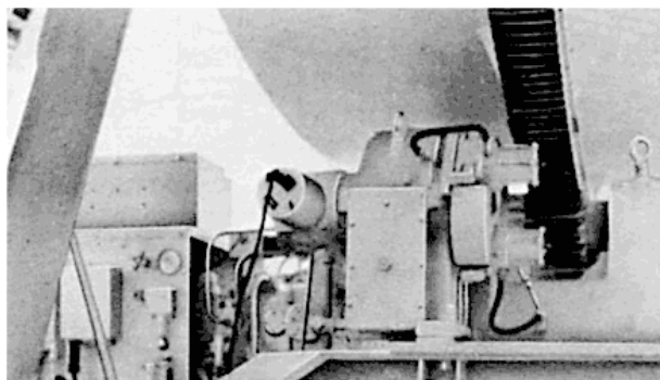
Figure 1—Photograph of USB antenna drive system showing X-bull gear and hydraulic motor.
