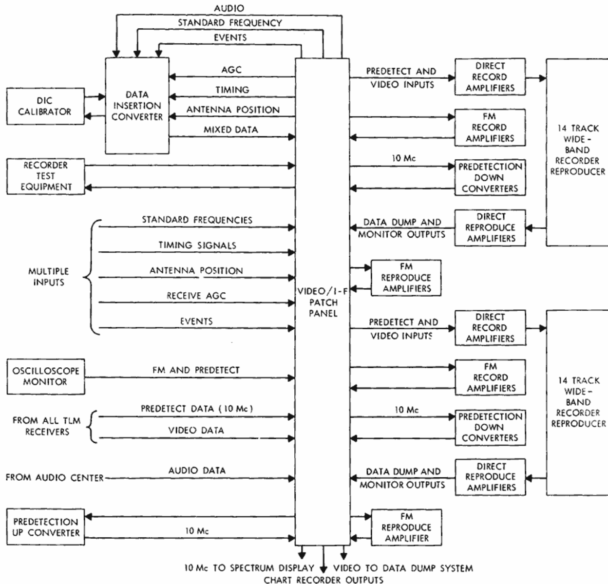
Figure 8—Video/IF distribution block diagram.
