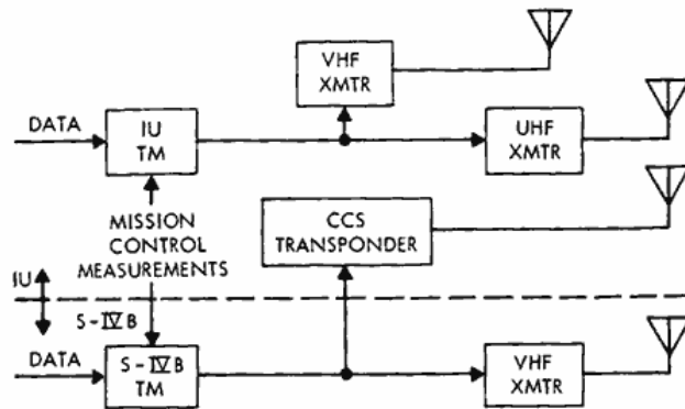
Figure 2—Telemetry systems.
