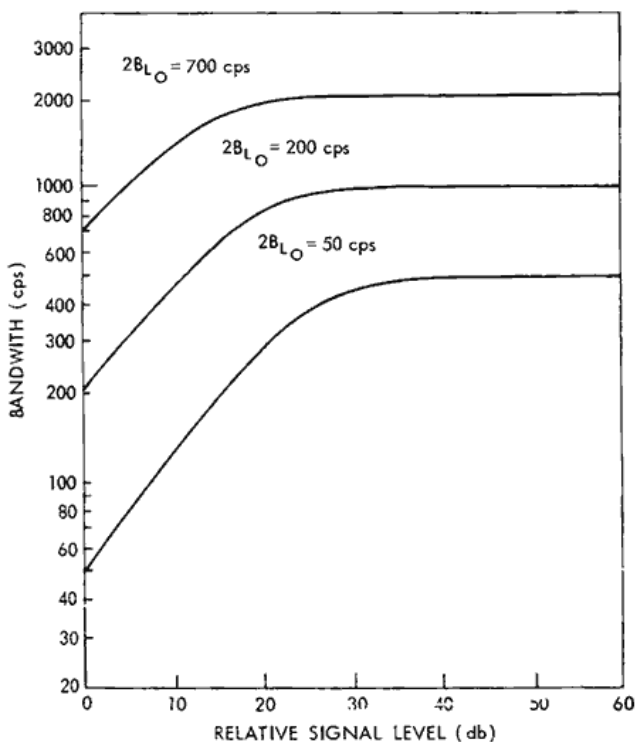
Figure 7—RF loop noise bandwidth as a function of relative signal level above RF design frequency threshold.
