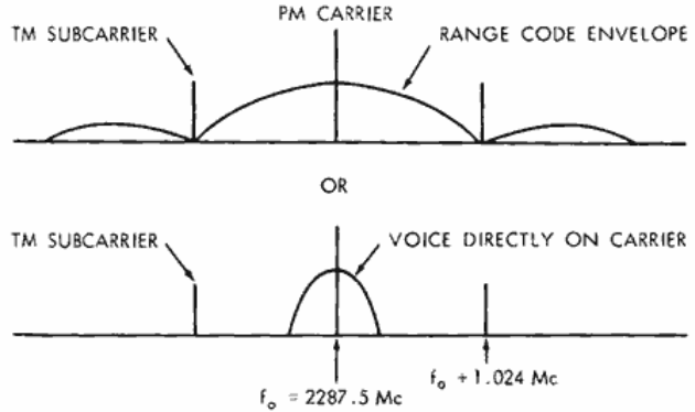
Figure 4—Contingency down-link spectrum.
