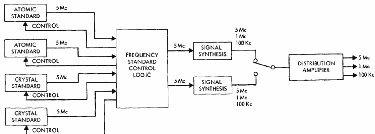
Figure 1—Apollo precision frequency source.
