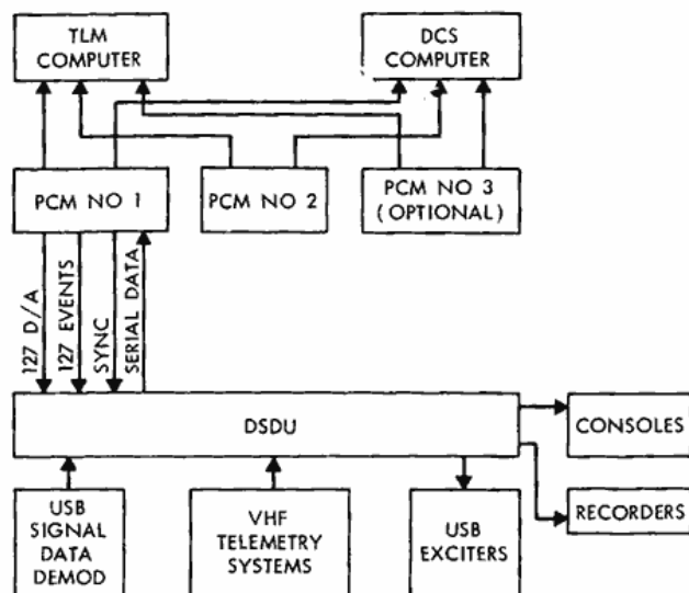
Figure 1—PCM system interface diagram.
