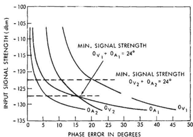
Figure 6—Phase errors for doppler dynamic conditions versus input signal level where 0_{V_1} and 0_{A_1} represent a frequency deviation ( f_d ) of \pm 181.5 kilocycles and a center frequency ( f ) of 63 kilocycles 2 , and where 0_{V_2} and 0_{A_2} represent an f_d of \pm 90 kilocycles and an f of 35 kilocycles 2 .
