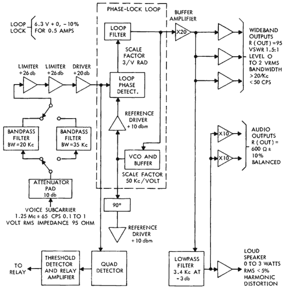
Figure 7—Voice subcarrier demodulator.
