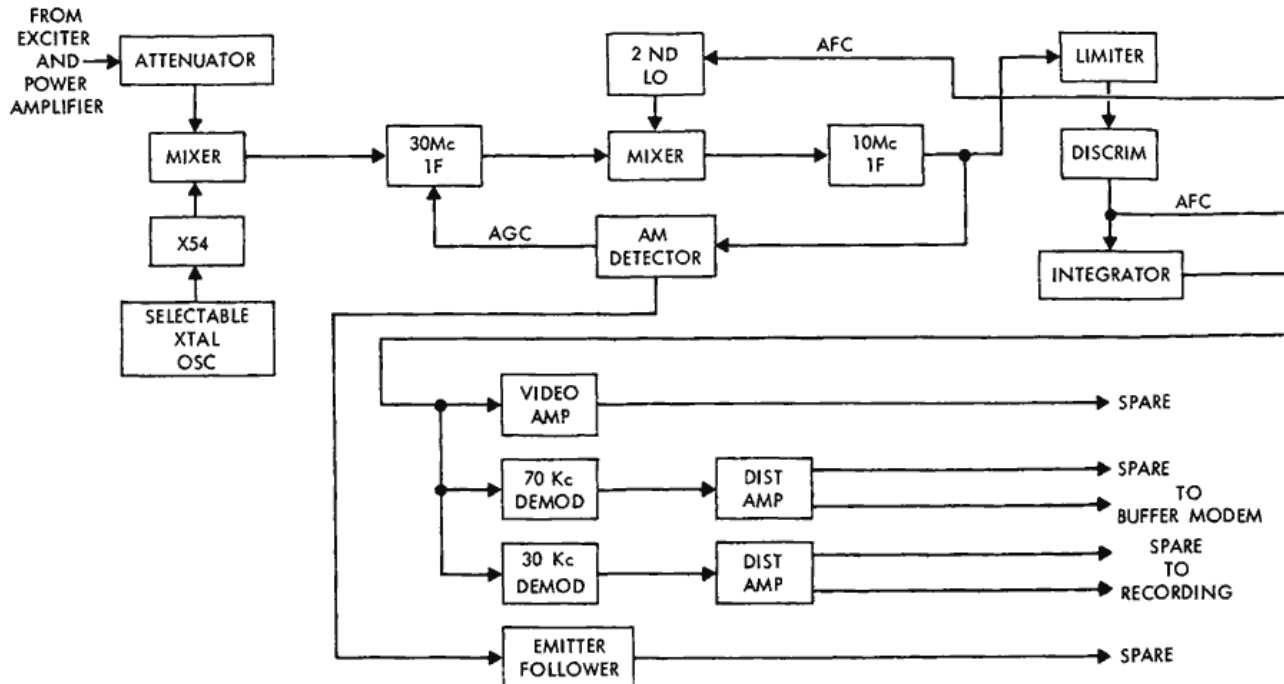
Figure 6—Verification receiver.
