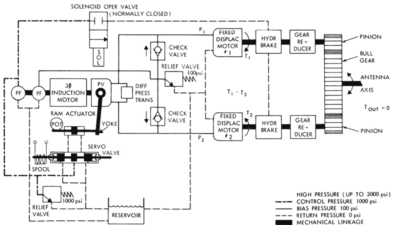
Figure 4—Schematic of hydraulic drive system with no excitation and brakes applied.
