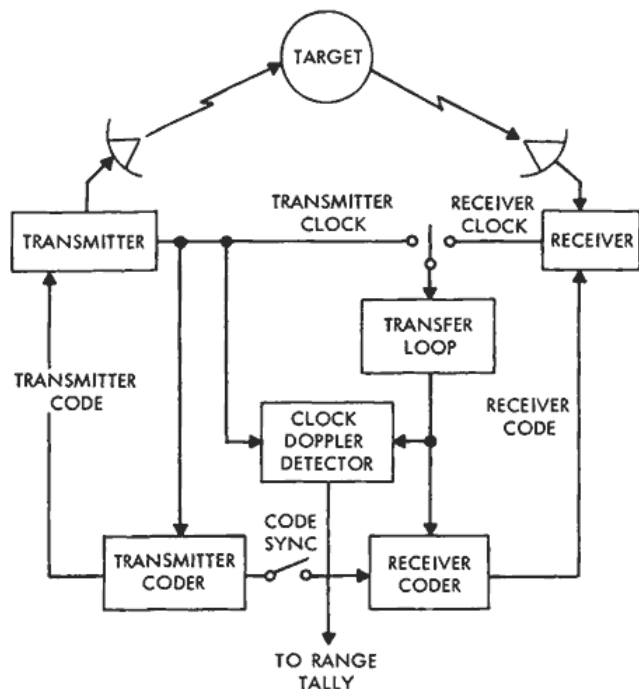
Figure 5—Phase modulation of S-band carrier.
