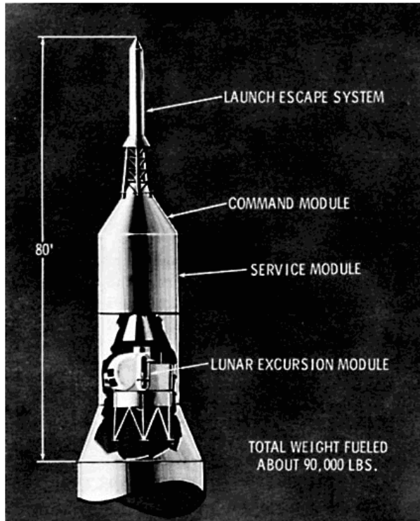
Figure 2—Apollo spacecraft.
