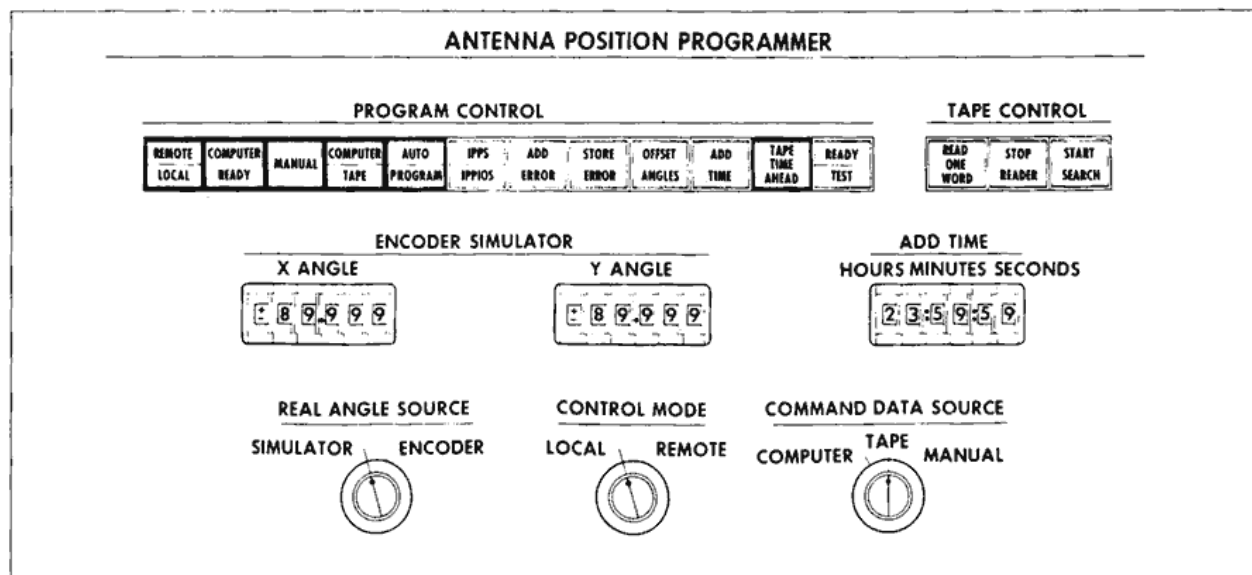
Figure 3—Antenna position programmer control panel (local).
