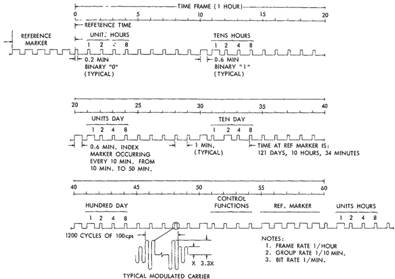
Figure 6—NASA 1/hour binary time code.
