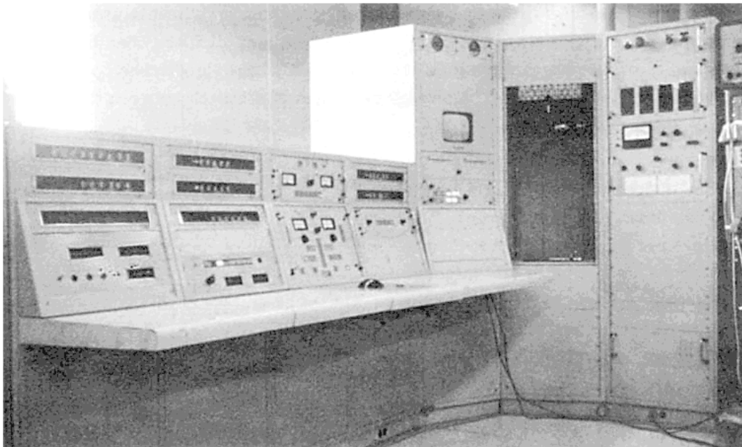
Figure 9—Complete operator's station.
