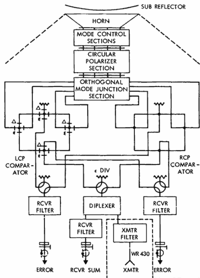
Figure 2—Cassegrainian feed system, block diagram.
