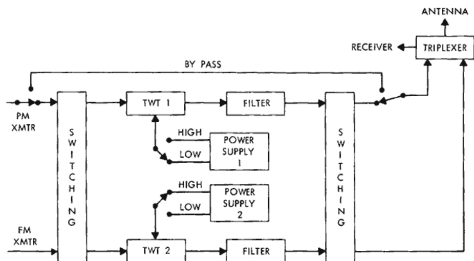
Figure 8—Diagram of CSM S-band power amplifier subsystem.
