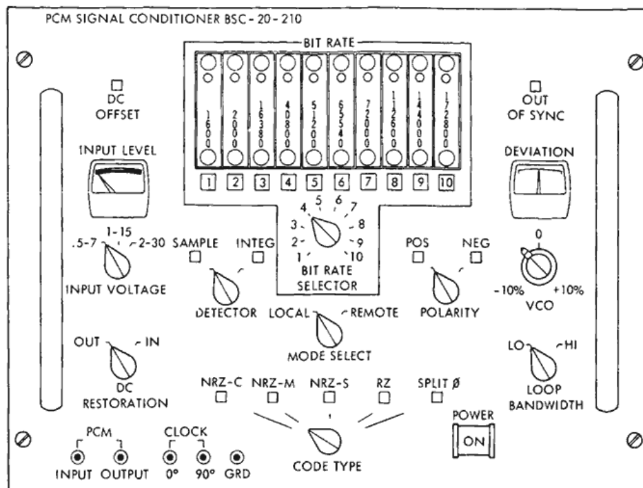
Figure 5—Narrow band bit synchronizer, front panel.
