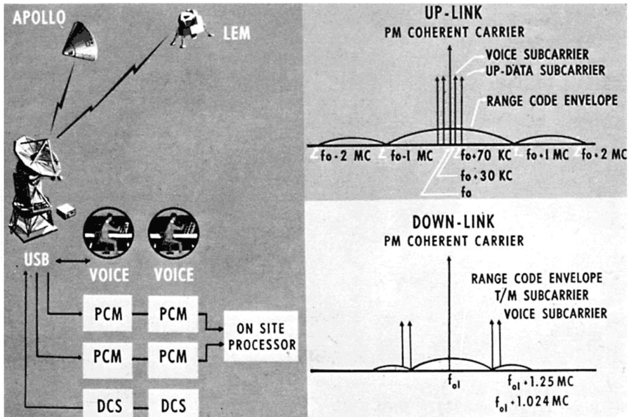
Figure 2—USB modulation technique.
