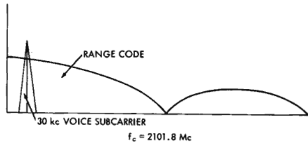
Figure 2—Full up-link PM spectrum.
