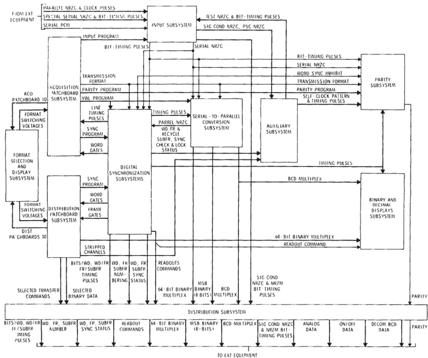
Figure 15—Patchboard PCM system.
