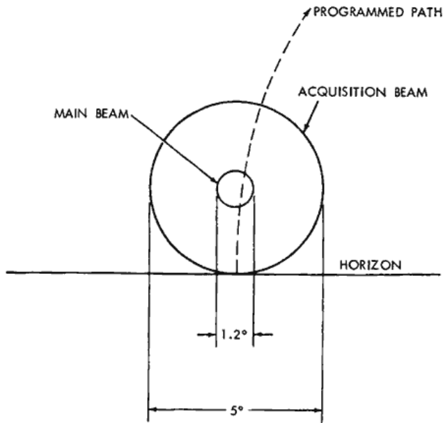
Figure 1—Ground transmit and receive pattern in space.
