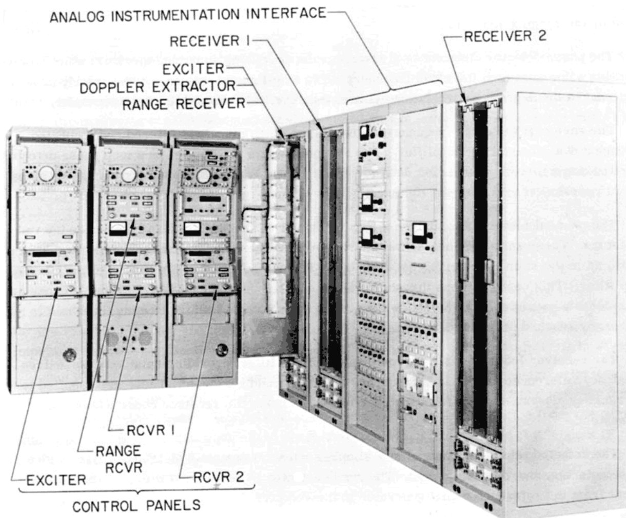
Figure 9—Receiver-exciter subsystem.
