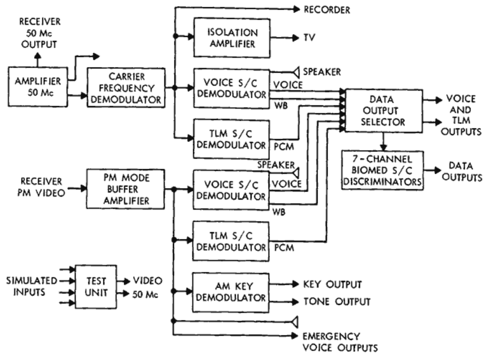
Figure 4—Signal data demodulator system.
