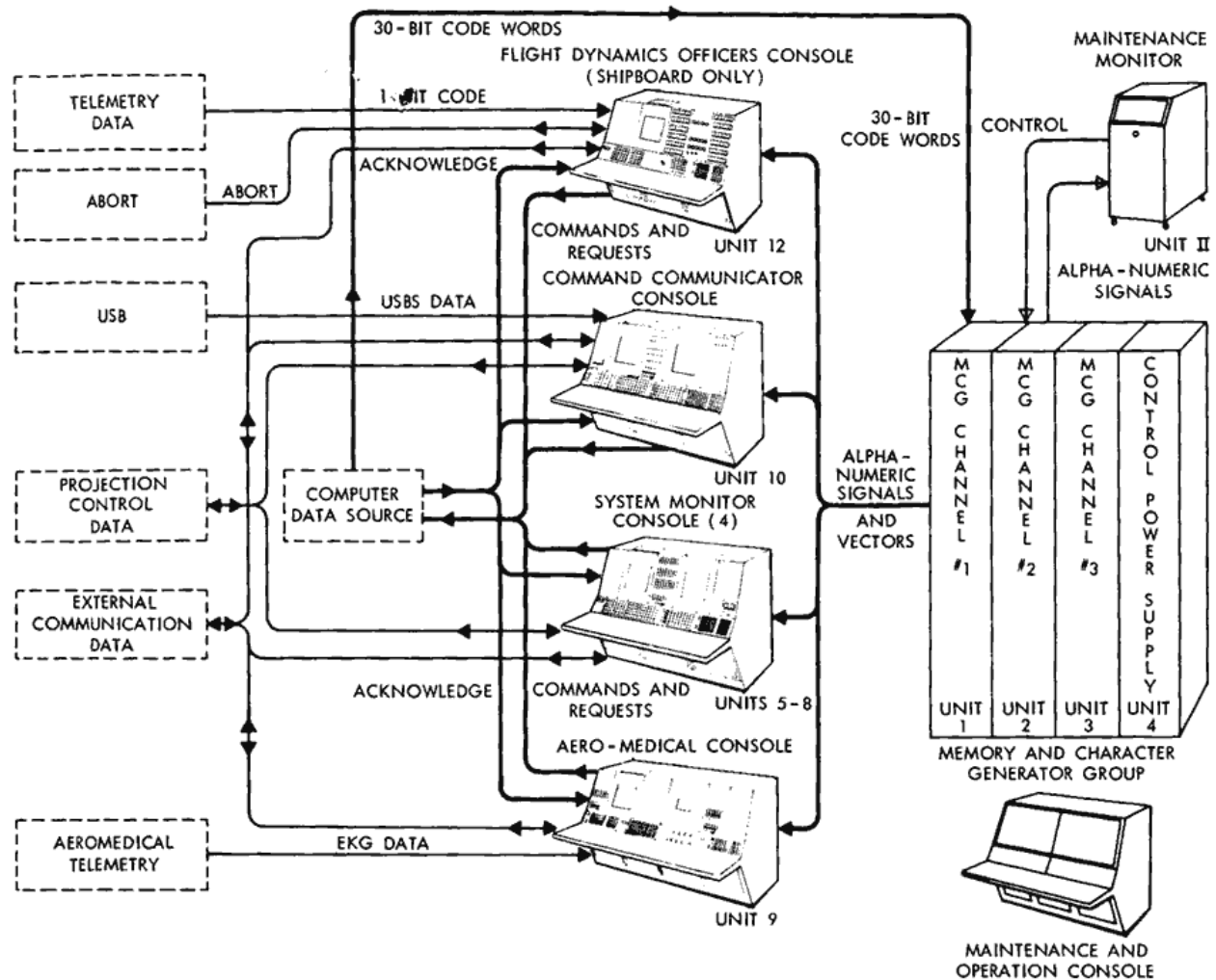
Figure 1—Display system for Apollo program.
