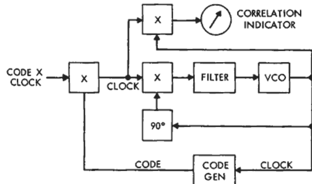
Figure 6—Double-loop code tracking system.
