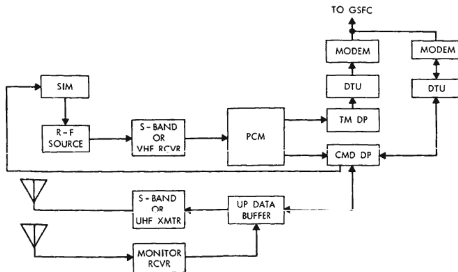
Figure 8—Typical remote site closed loop test block diagram.
