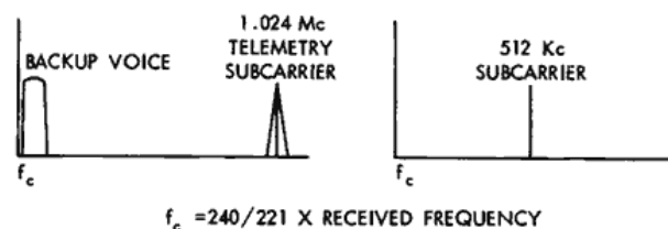
Figure 4—Down-link RF spectra for contingency modes (PM).
