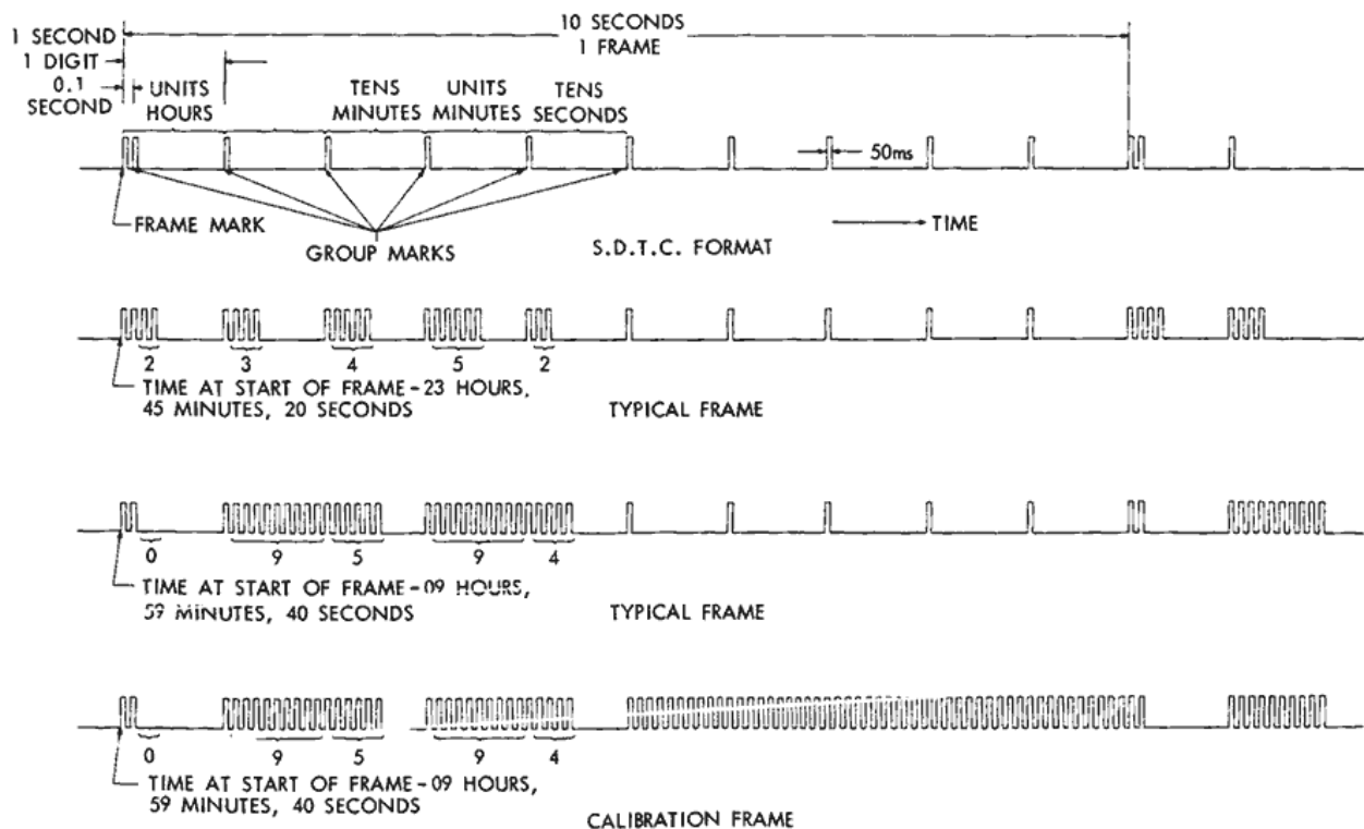
Figure 7—Format serial decimal time code.
