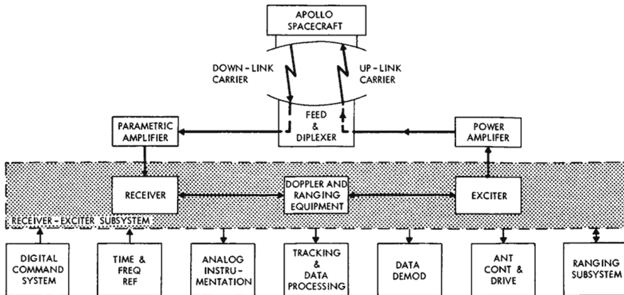
Figure 1—Receiver-exciter Unified S-Band system functions: doppler extraction, two-way communications, angle tracking and ranging.
