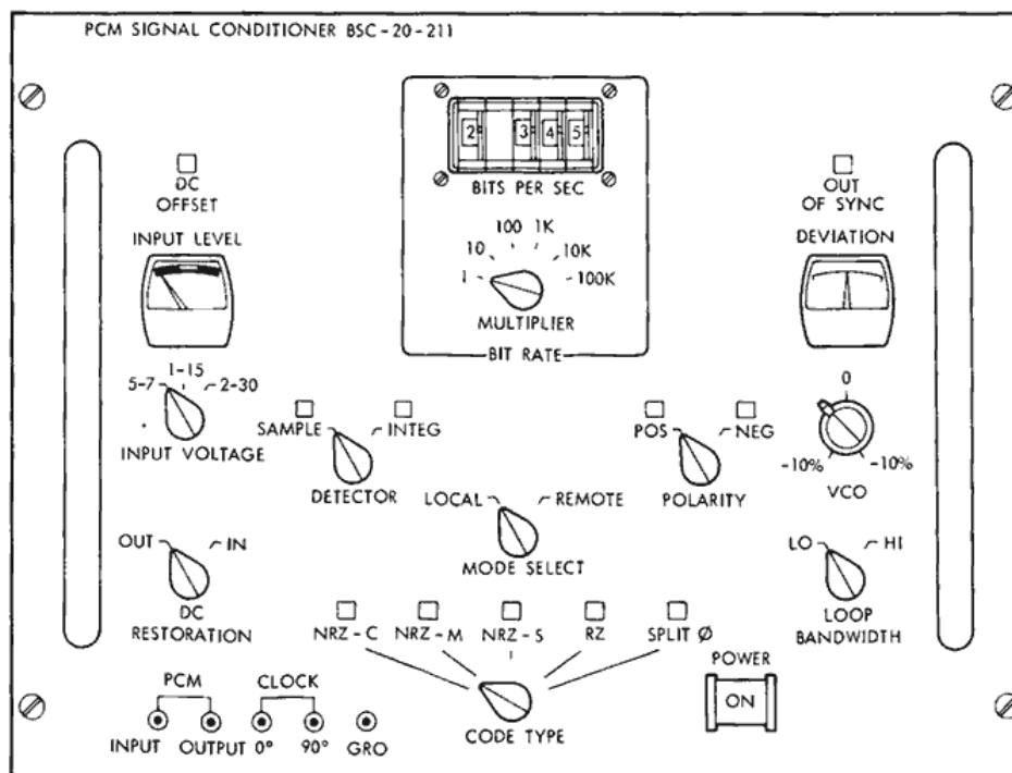
Figure 6—Wide band bit synchronizer, front panel.
