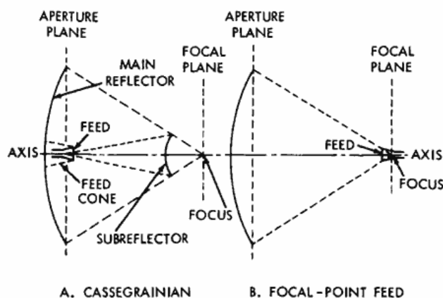
Figure 1—Antenna feed systems.
