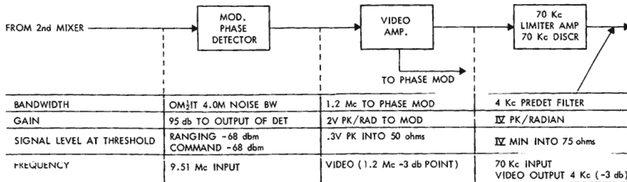
Figure 4—Gain, bandwidth power distribution.
