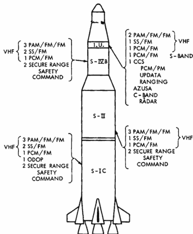
Figure 1—Saturn V instrumentation systems.
