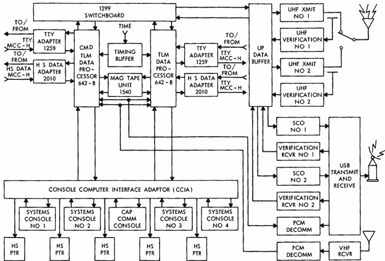
Figure 2—Apollo digital command system.
