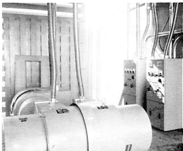
Figure 8—Motor-generator.
