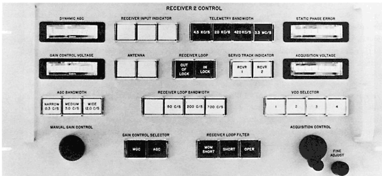
Figure 11—Receiver 2 control.
