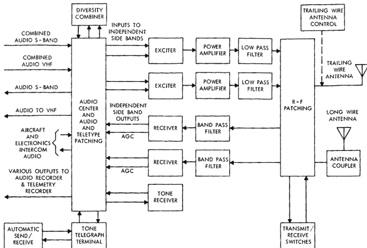
Figure 9—Aircraft/ground communications block diagram.
