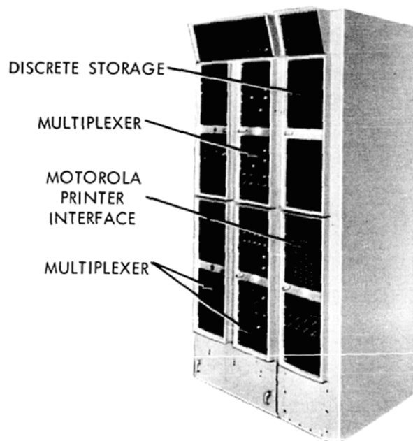
Figure 6—Console computer interface adapter.
