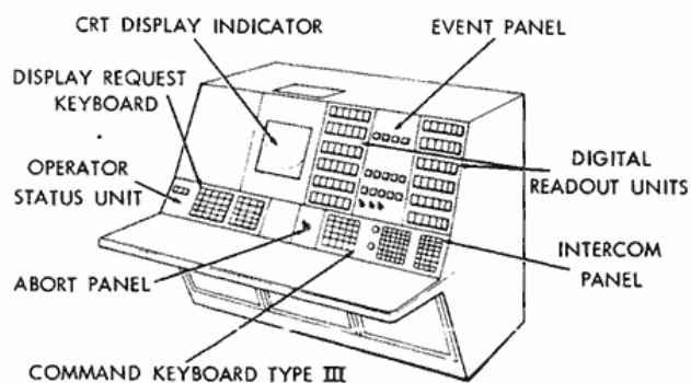
Figure 18—Flight dynamics officer's console.
