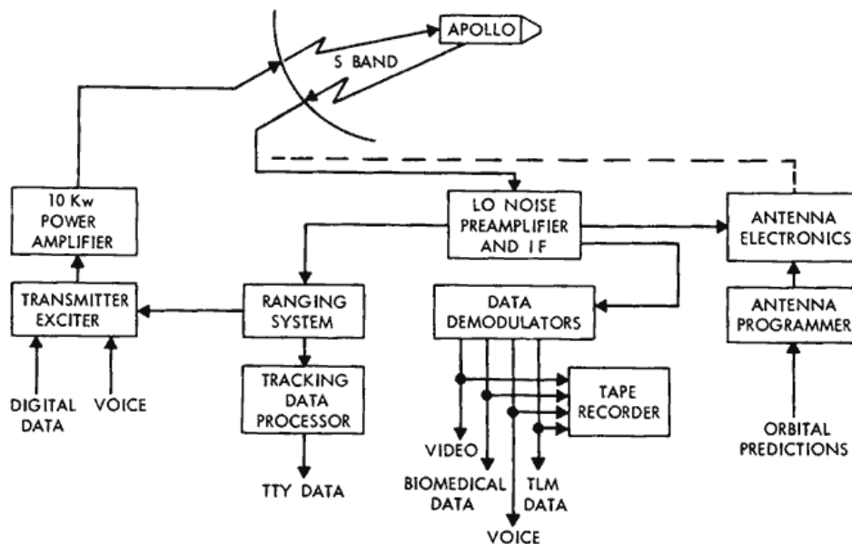
Figure 3—Simplified Apollo Unified S-Band system.
