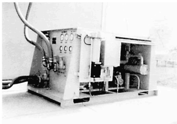
Figure 7—Liquid-to-air heat exchanger for use in ships' systems.
