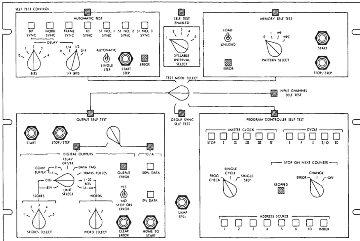
Figure 9—Self-test control panel.
