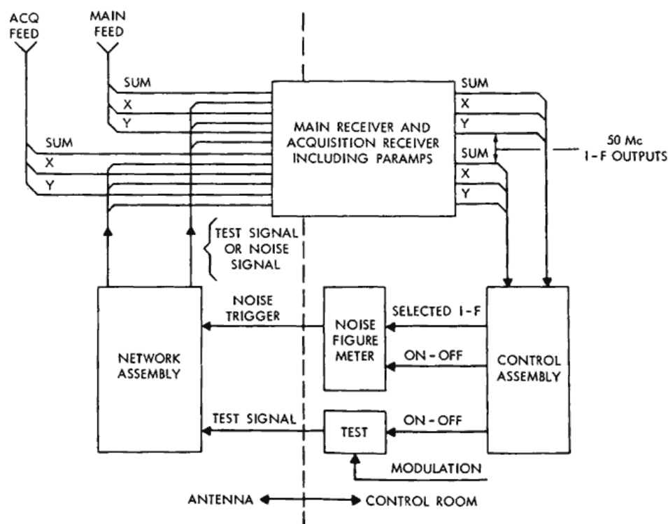
Figure 1—Functional block diagram of noise figure and test signal injection subsystem.
