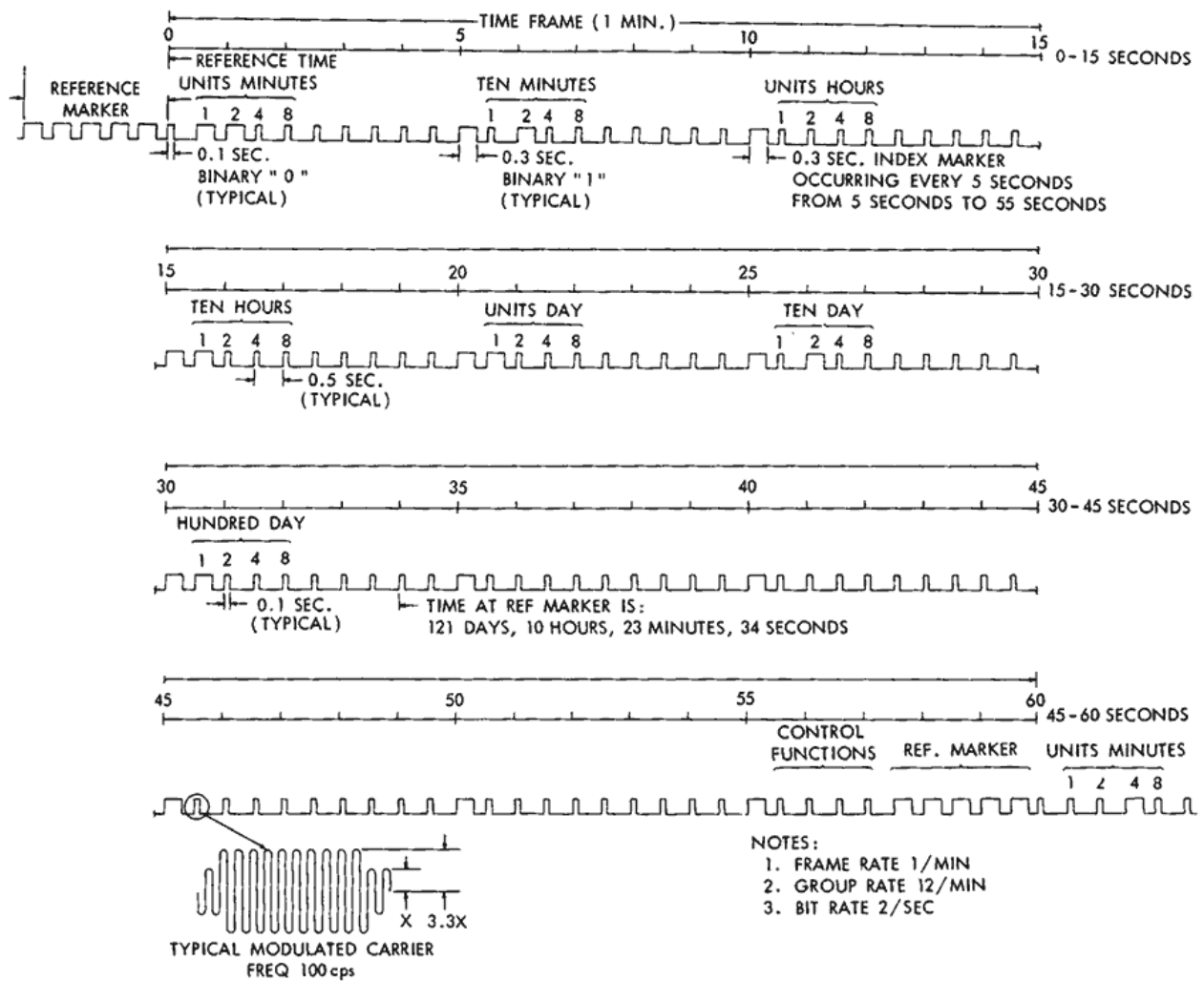
Figure 5—NASA 1/minute binary time code.
