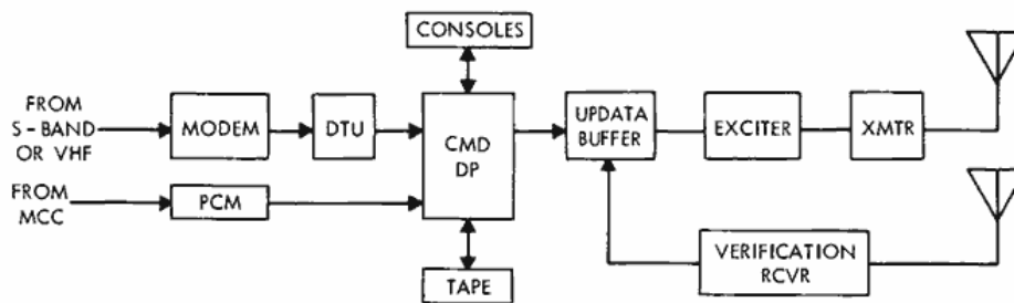
Figure 4—Uplink data block diagram.
