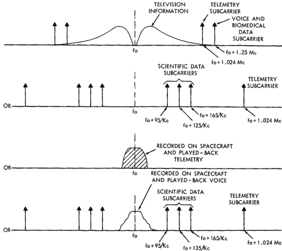
Figure 2—FM spectra of frequency modulated carriers.
