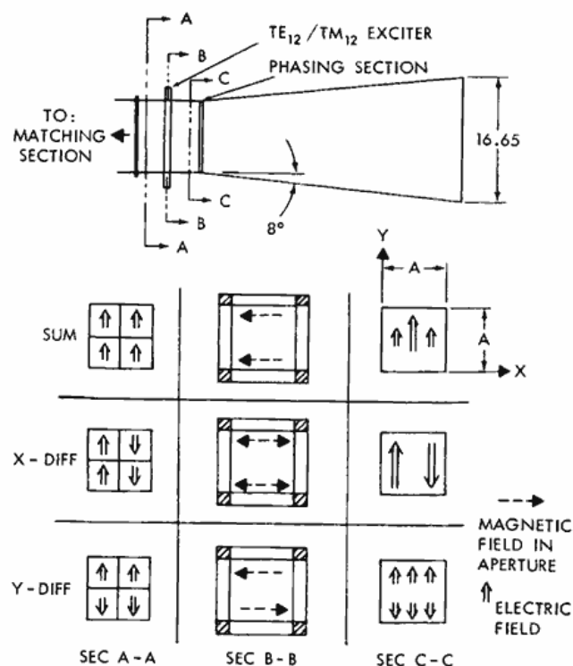
Figure 3— TE_{12}/TM_{12} exciter.
