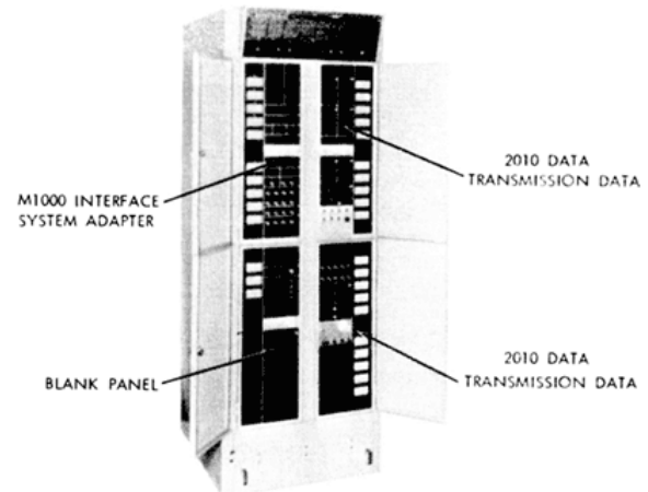
Figure 5--Peripheral communications system.
