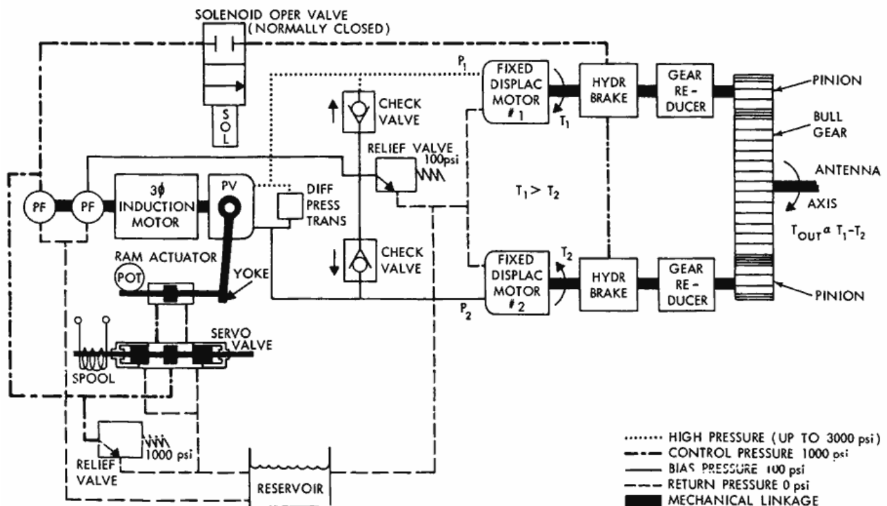
Figure 5—Schematic of hydraulic drive system with brakes lifted and signal applied to servo valve causing its spool to be displaced to right.
