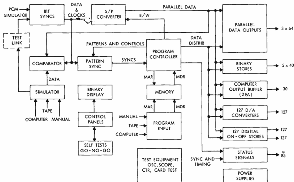
Figure 4—Block diagram of stored program PCM data decommutation system number 6000.
