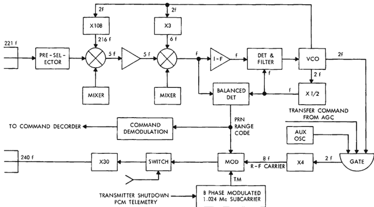
Figure 3—Transponder block diagram (ABC loop not shown).
