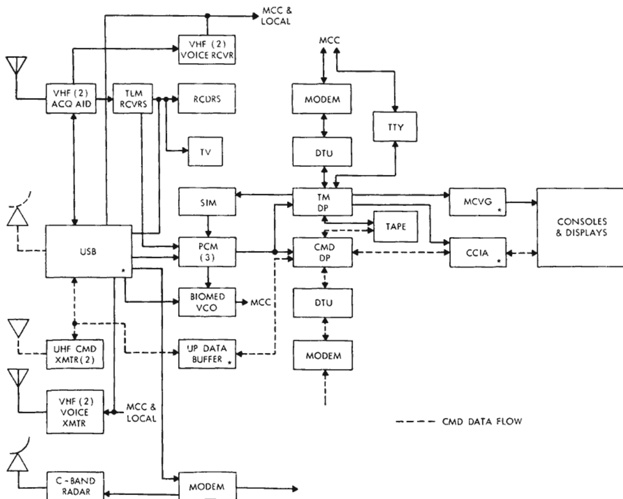
Figure 3—Typical remote site command data flow block diagram.
