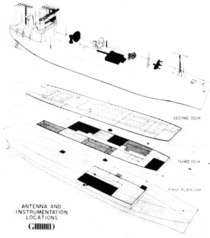
Figure 10—Location of instrumentation systems on ship providing insertion/injection coverage.
