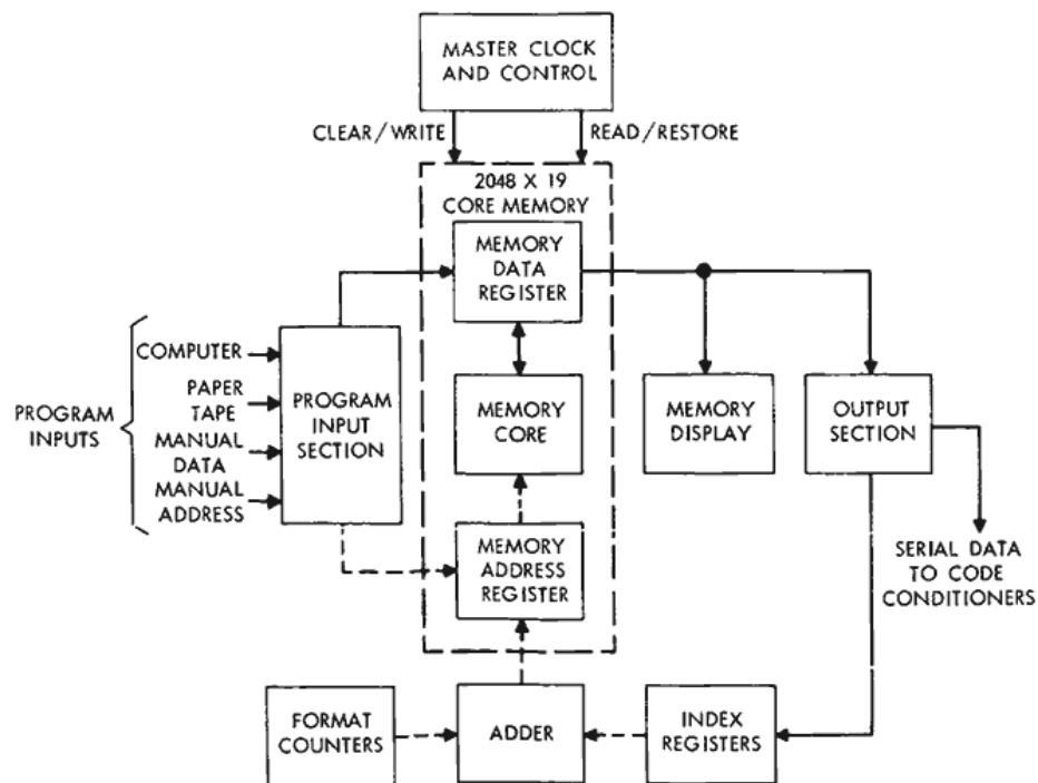
Figure 10—Block diagram of PCM stored program simulator.
