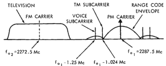
Figure 2—Typical down-link spectrum.
