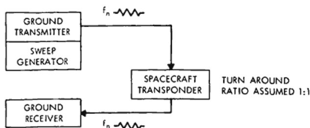
Figure 2—Diagram illustrating procedure for two-way RF acquisition.
