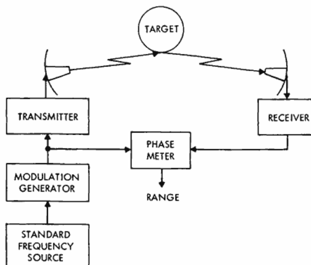
Figure 1—CW radar ranging system.
