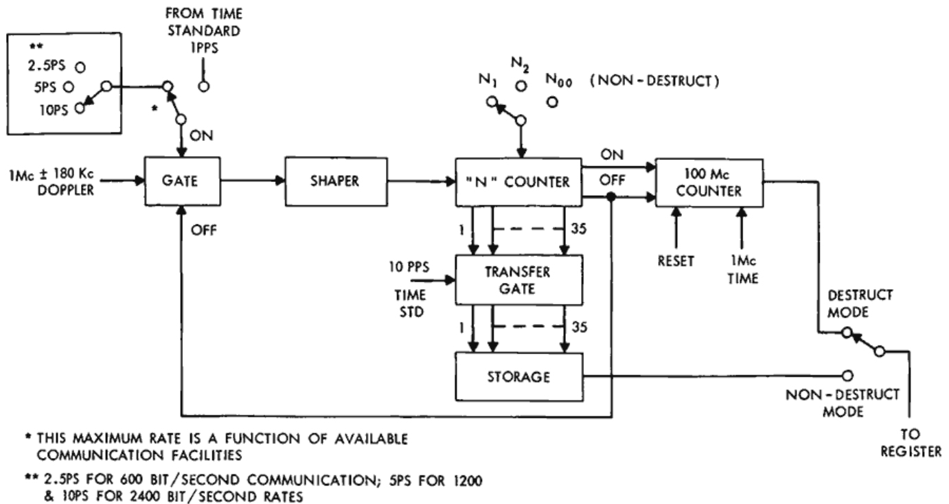
Figure 11—Shipboard doppler counter.
