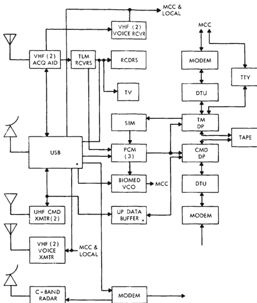
Figure 6—Typical remote site block diagram without consoles.
