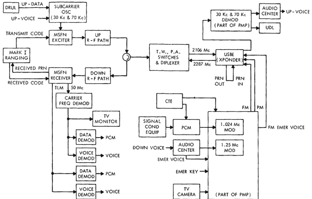
Figure 1—Block I system test configuration.
