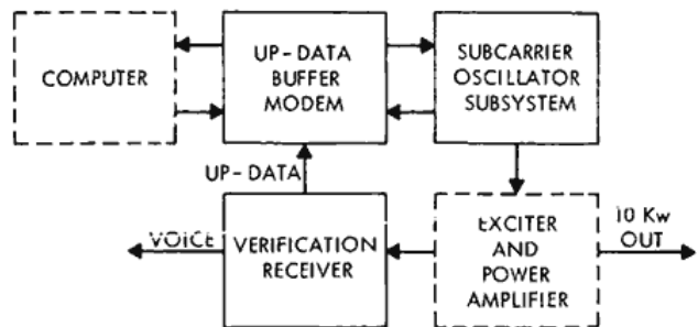
Figure 1—Relationship between up-data buffer modem, subcarrier oscillator subsystem, and verification receiver.
