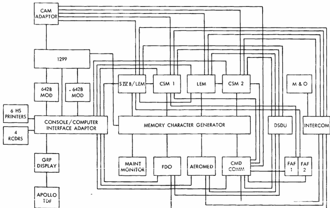
Figure 2—Apollo display and interface external signal cabling diagram.
