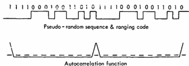
Figure 4—Pseudo-random binary sequence and ranging code waveform.
