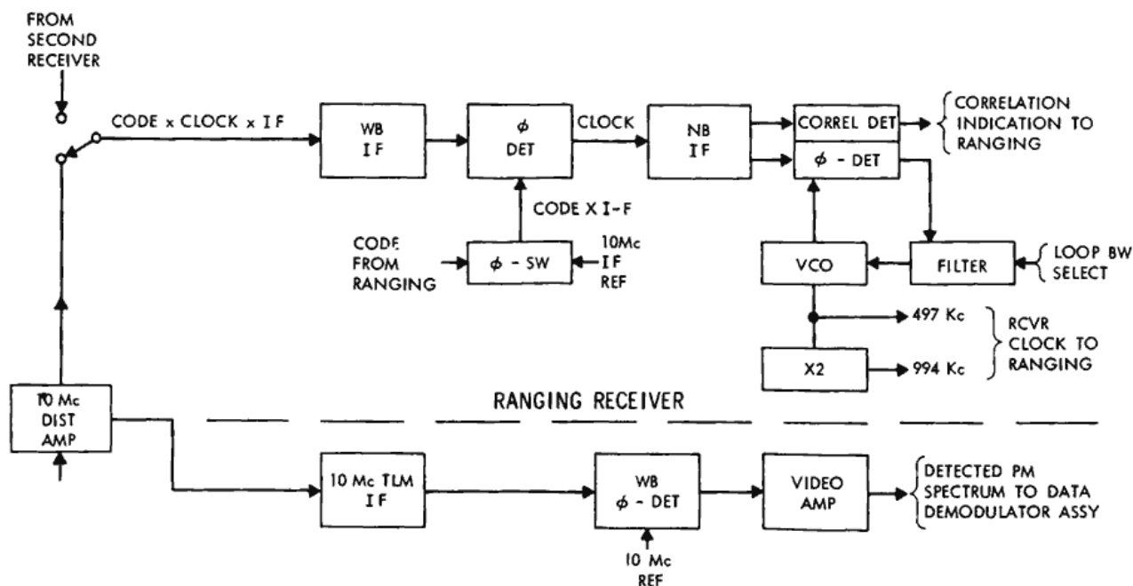
Figure 8—Detected telemetry channel (typical).
