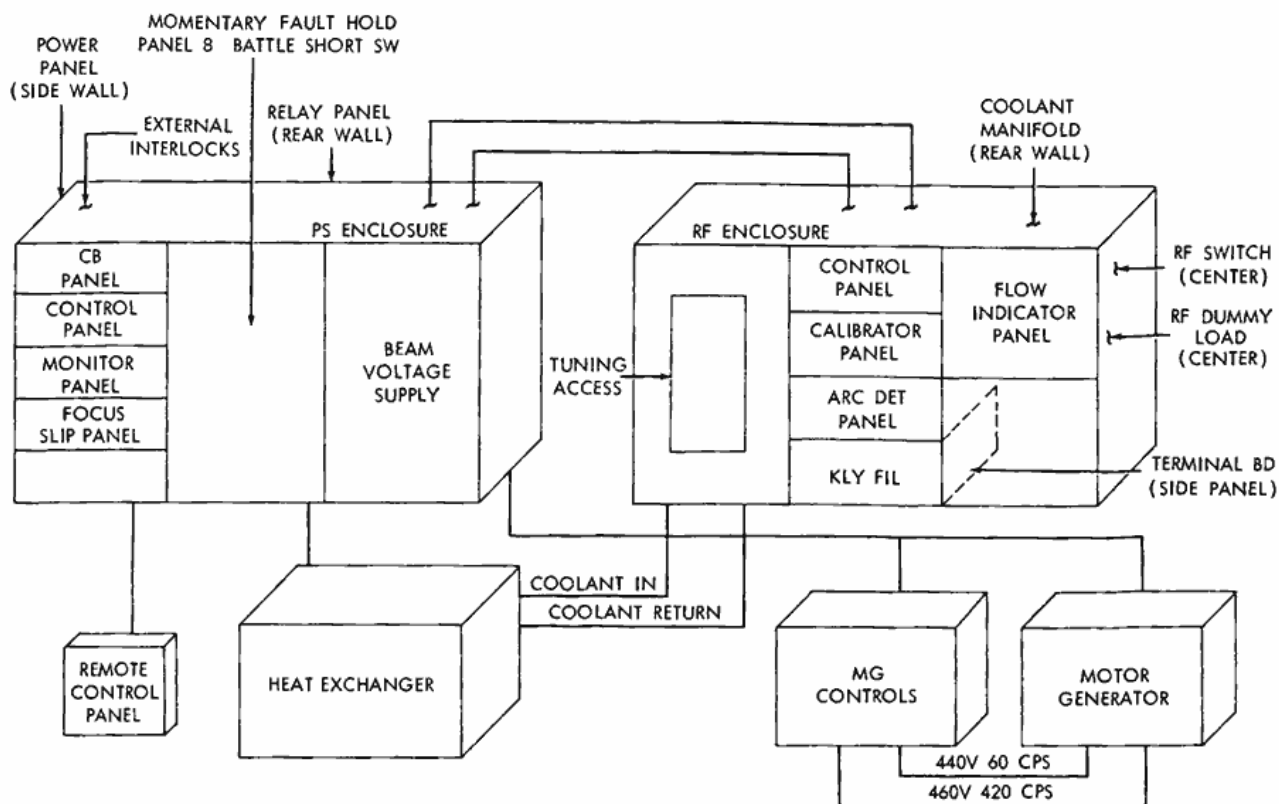
Figure 2—Power amplifier unit identification.
