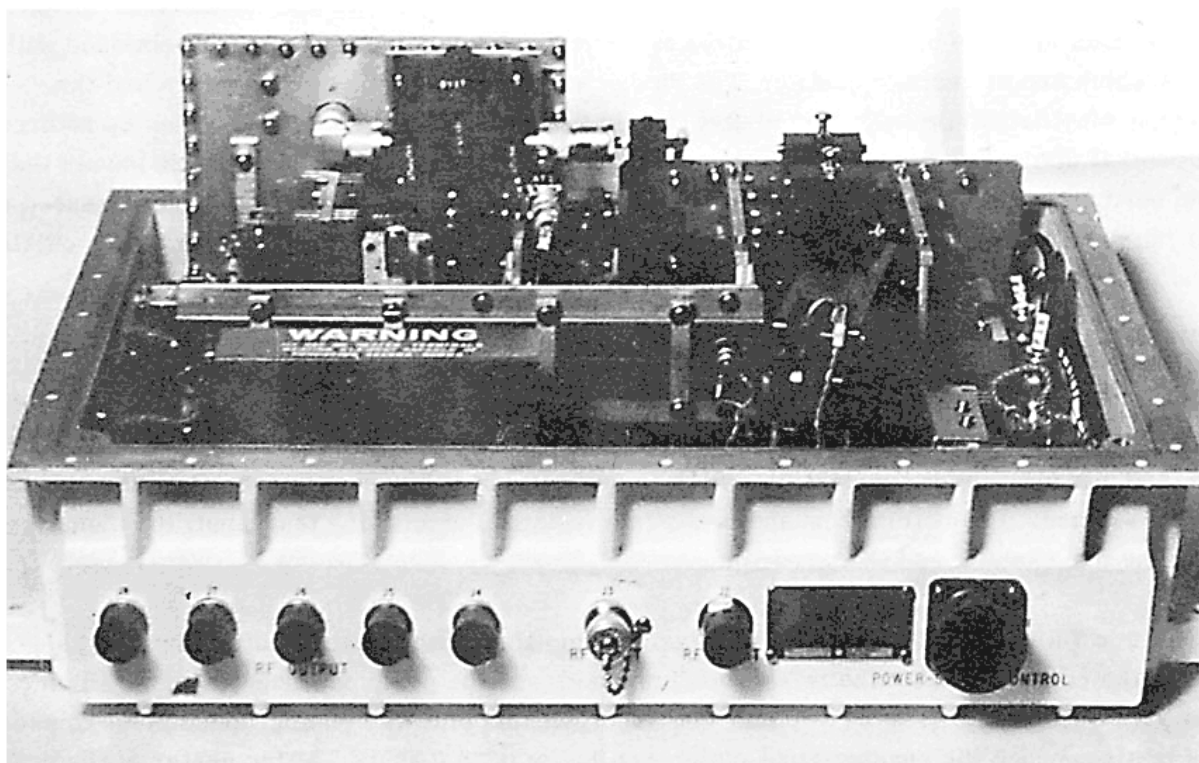
Figure 7—Parametric amplifier, enclosure removed.
