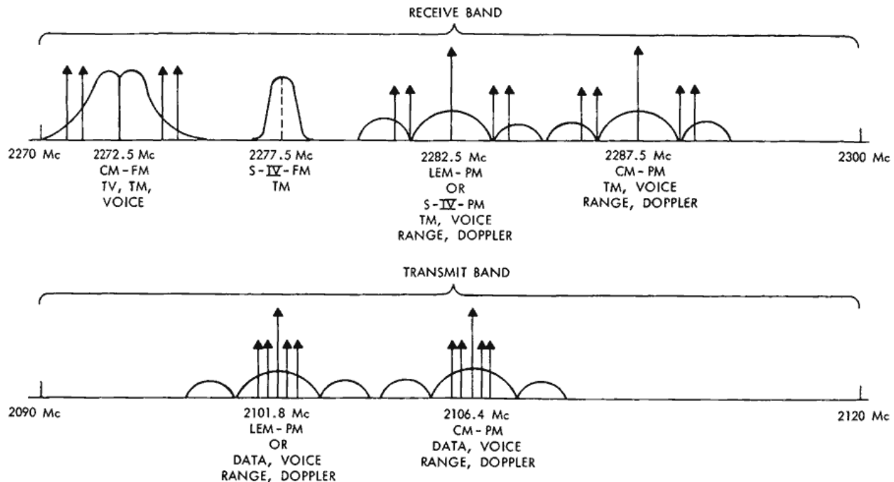
Figure 3—USB system frequency spectrum.
