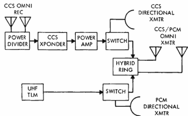
Figure 6—Antenna system.
